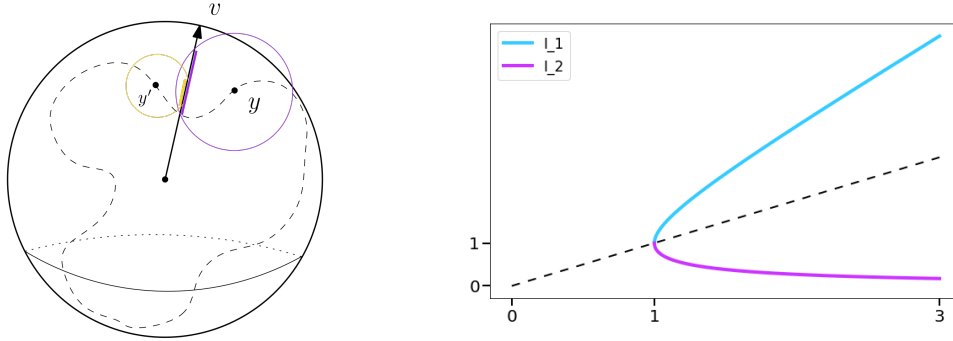
Figure 38: Left: Representation of two intervals \langle v \rangle_+ \cup \overline{B}(y, t) and \langle v \rangle_+ \cup \overline{B}(y', t) . Right: Representation of the maps x \mapsto x \pm \sqrt{x^2 - 1} .
