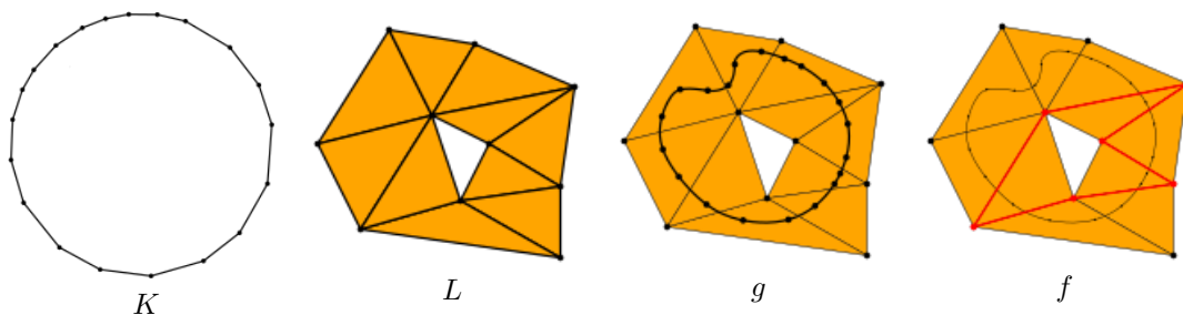
Figure 21: The map f (in red) is a simplicial approximation to g .
