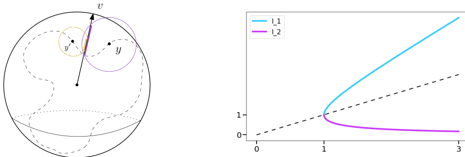
Figure 33: Left: Representation of two intervals \langle v \rangle_+ \cup \bar{\mathcal{B}}(y, t) and \langle v \rangle_+ \cup \bar{\mathcal{B}}(y', t) . Right: Representation of the maps x \mapsto x \pm \sqrt{x^2 - 1} .
