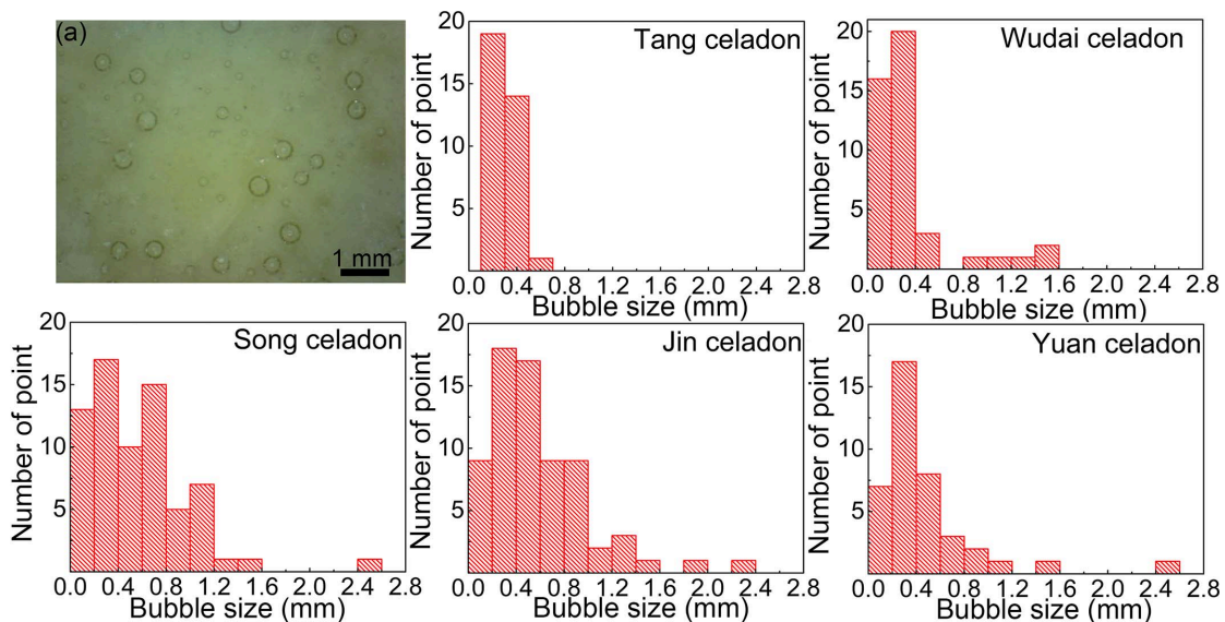
Fig. 2 Bubble observation of Tang celadon (sample number: YX-01-005) (a) and histograms of bubble size distribution for Tang, Wudai, Song, Jin and Yuan productions.
