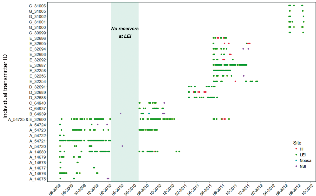
Fig. 4. Chronology of daily visitation patterns across all receivers deployed along the east coast of Australia (HI: Heron Island, LEI: Lady Elliot Island, Noosa: Noosa Heads, NSI: North Stradbroke Island, see Fig. 1c) for 33 tagged reef manta rays Mobula alfredi . Letters in front of the transmitter ID correspond to tagging campaign (A: June 2009, B: March 2010, C: June 2010, D: February 2011, E: June 2011, G: June 2012)
