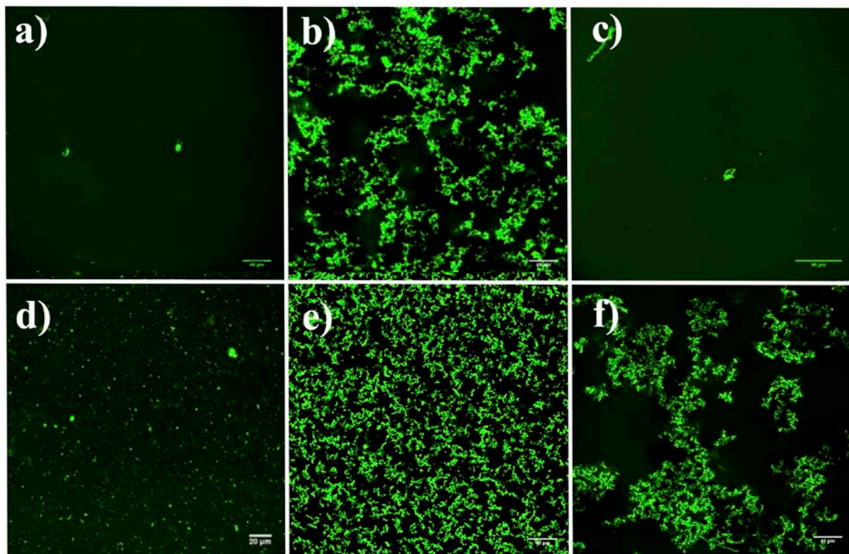
Figure 5. Fluorescence microscopy images (green channel) captured after incubation at 37 °C for: a) 31.2 \mu\text{M} RCA 120 -Fluorescein, b) 31.2 \mu\text{M} RCA 120 -Fluorescein/200 \mu\text{M} ELP( Gal ), c) 31.2 \mu\text{M} RCA 120 -Fluorescein/200 \mu\text{M} ELP( Glc ), d) 31.2 \mu\text{M} RCA 120 -Fluorescein in 10 % serum, e) 31.2 \mu\text{M} RCA 120 -Fluorescein/200 \mu\text{M} ELP( Gal ) in 10% serum, f) 31.2 \mu\text{M} RCA 120 -Fluorescein/200 \mu\text{M} ELP( Gal ) in 100 % serum.
