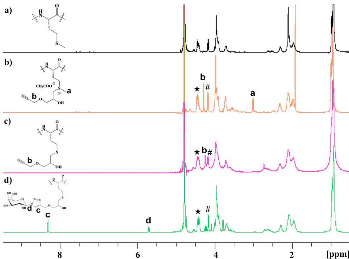
Figure 1. ^1\text{H} NMR spectra of a) ELP, b) ELP( Alkyne ), c) ELP( Dem Alkyne ) and d) ELP( Gal ) in \text{D}_2\text{O} at 25^\circ\text{C} . Resonance # corresponds to Val \alpha\text{CH} of the guest residue in \text{VPGY}\underline{\text{G}} repeat units, and resonance \star corresponds to Val \alpha\text{CH} and Pro \alpha\text{CH} of \underline{\text{V}}\text{PGXG} repeats.
