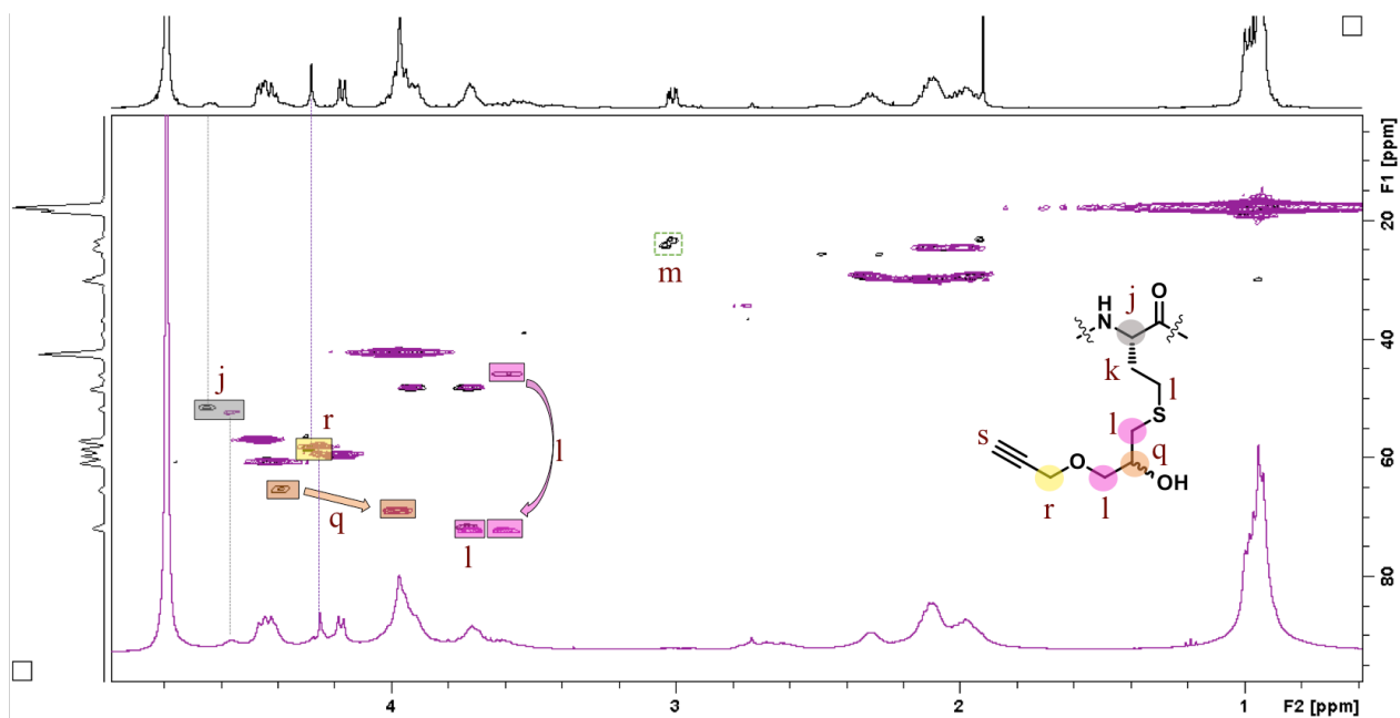
Figure S5. HSQC spectra of ELP(Alkyne) (in black) and b) ELP(Dem Alkyne) (in pink) in D 2 O at 25 °C.
