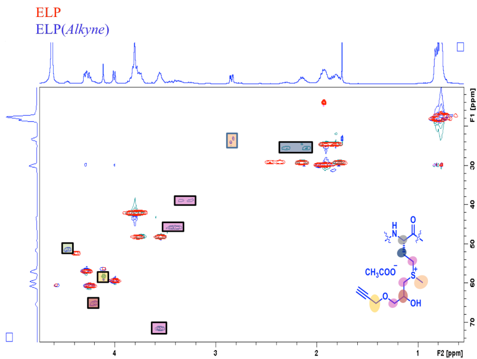
Figure S2. ^1\text{H-NMR} spectrum of ELP( Alkyne ) in \text{D}_2\text{O} at 25^\circ\text{C} .
