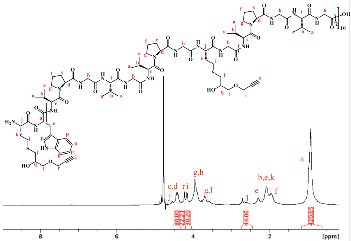
Figure S4. 1 H-NMR spectrum of ELP(Dem Alkyne) in D 2 O at 25 °C.
