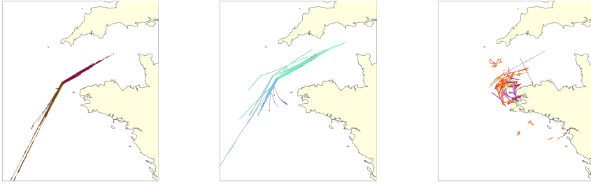
Fig. 10 50 trajectories of three estimated trajectory clusters, see the text for details. Colors correspond to those of Fig. 9.
