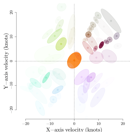
Fig. 9 Movement modes estimated distributions (on the velocity space). Each ellipsoid represents a movement mode distribution, the dot being the expected mean, and the contour the 50% centered quantile. The transparency shows the estimated relative weight. The dotted lines show the 0 values.
