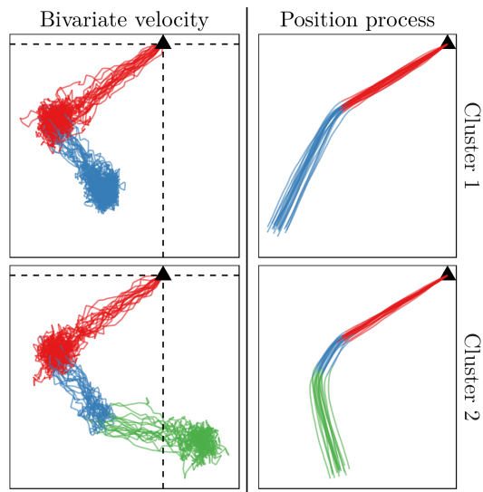
Fig. 7 Simulated trajectory data. Three movement modes are shared by two clusters. Each cluster corresponds to two different routes. The black triangle denotes the beginning of each trajectory. The first two movement modes are present in both clusters.
