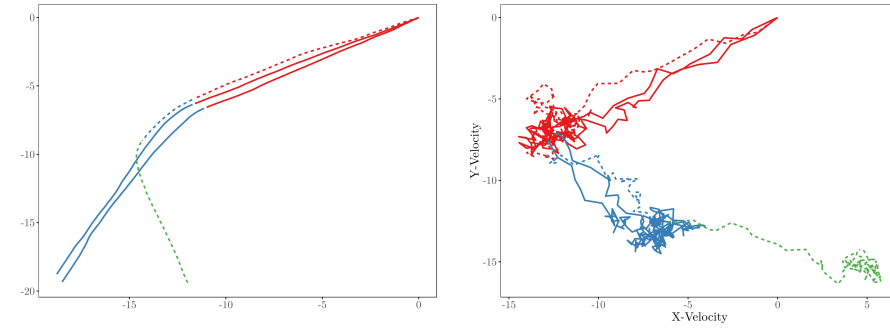
Fig. 4 Simulation of three different trajectories with the same model as in Figure 3. The left panel shows the position processes, the right panel shows the velocity processes. All processes start from (0, 0) . (Left) Two trajectories (in plain lines) are made of the same movement modes so they belong to the same cluster. The other trajectory (dashed line) has a different distribution over movement modes so it belongs to another cluster. (Right) The trajectories are plotted on the bivariate velocity space, showing the three possible movement modes. Two of them (red and blue) are shared by the two trajectory clusters.
