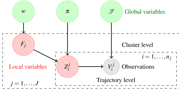
Fig. 6 Graphical representation of the hierarchical structure of the simplified model of Section 3.1.
