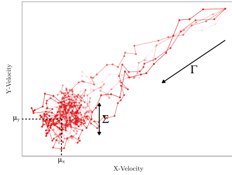
Fig. 2 Five realizations of bivariate Ornstein Ulhenbeck Processes of parameters \mu , \Gamma and \Sigma , solution of the SDE eq.(1), starting at position v_0 = (0, 0) (top right corner).
