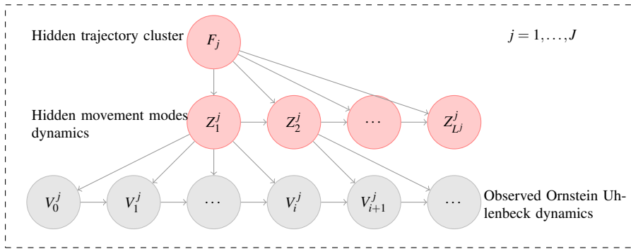
Fig. 5 Modelling framework for the two level clustering of our movement data set (consisting in J trajectories). Equations for the Ornstein-Uhlenbeck dynamics are given in section (2). Hidden movement mode dynamics are not fully specified, as a simplified independent model will be used for inference. Classical modelling framework would be a Markov chain or a semi Markov chain. Notations used in this Figure are detailed in Section 3.
