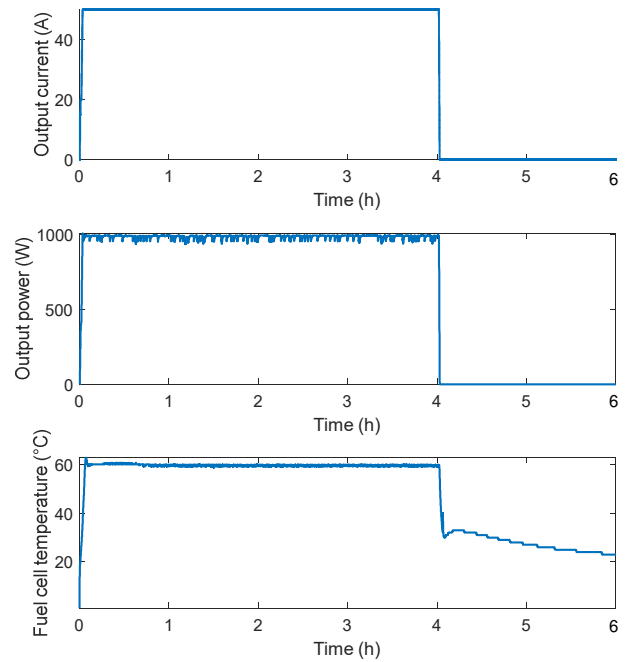
Figure 6: cycling profile
