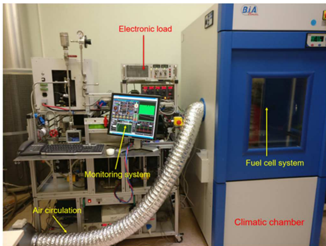
Figure 5: Test bench
