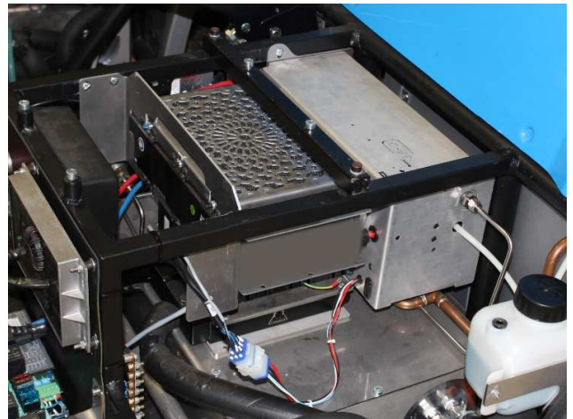
Figure 4: Fuel cell system
