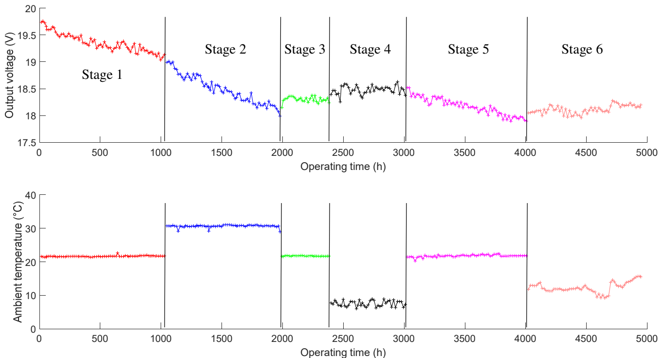
Figure 1: Evolution of system output voltage all along the experimentation
