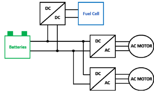
Figure 3: Mobypost vehicle architecture
