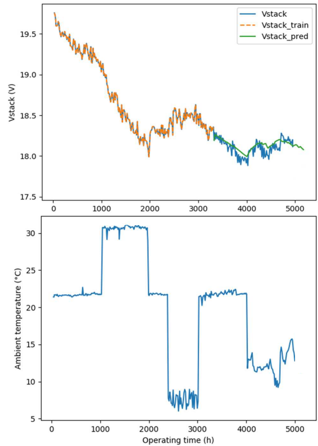
Figure 9: Results with learning rate = 60%
