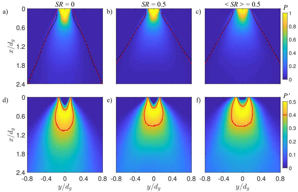
Figure 9: (color online) Probability (average of the thresholded image stack) of liquid presence (a-c) and its variations (standard deviation of the thresholded image stack) (d-f). The columns corresponds to M = 25 and SR = 0 (a, d), M = 25 and SR = 0.5 (b, e) and \langle M \rangle = 25 and \langle SR \rangle = 0.5 (c, f). a-c) The black dots and red dashed lines define the spray edge and initial angle (see Figure 5); d-f) The red line is a contour of the liquid presence variations being equal or higher than 0.4.
