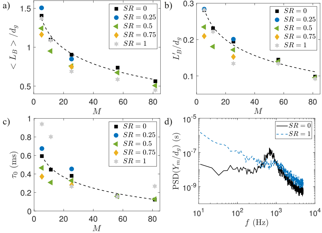
Figure 7: (color online) Evolution of the liquid core length mean \langle L_B \rangle (a), standard deviation L'_B (b) and timescale \tau_0 (c) as a function of the momentum ratio M , for different swirl ratios SR . The dashed lines are fits along M for SR = 0 of values \langle L_B \rangle = 1.85 \pm 0.22 - (0.29 \pm 0.07) \log(M) , L'_B = 0.39 \pm 0.05 - (0.06 \pm 0.02) \log(M) and \tau_0 = 0.89 \pm 0.17 - (0.17 \pm 0.05) \log(M) . d) Raw PSD of the y coordinate of the center of area of the liquid core Y_m for M = 80 , SR = 0 (with a peak around 700 Hz) and SR = 1 .
