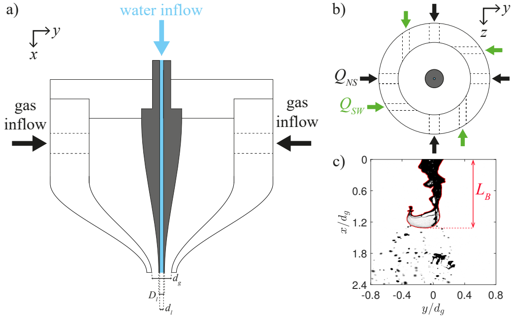
Figure 1: (color online) Longitudinal (a) and transverse (b) cuts of the coaxial two-fluid atomizer (the complete 3D geometry is open-source and available at http://depts.washington.edu/fluidlab/nozzle.shtml ). Water is injected in the center of the atomizer, while gas enters the nozzle through 8 inlets in a horizontal plane. It then flows along the cubic-spline-shaped walls inside the atomizer. Four inlets are on the atomizer's axis and produce a longitudinal gas co-flow while four others are off-axis and induce angular momentum in the gas jet produced at the exit of the atomizer. The atomizer axis is vertical, pointing downward, and is denoted x . c) Back-lit image of the spray for M = 5.3 and SR = 0 , covering a field of view of 2.4 \times 1.6 d_g^2 , with a resolution of 2.7 \cdot 10^{-3} d_g ( 27 \mu\text{m} ). The camera axis z is perpendicular to x , yielding images in the longitudinal plane (x, y) . The image was background-corrected and the grayscale goes from 0 to 1. The red contour correspond to the liquid core and is obtained through image processing; its longitudinal extent defines the liquid core length L_B .
