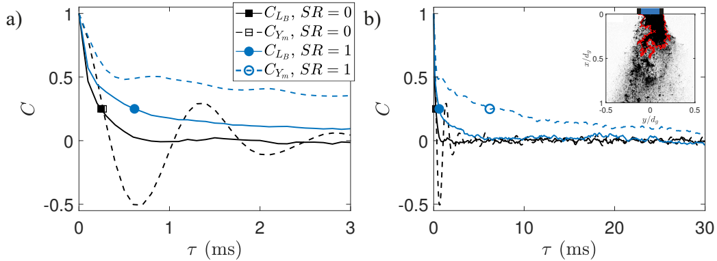
Figure 8: (color online) Auto-correlation function of both the liquid core length L_B (filled marker) and the y coordinate of the center of area of the liquid core Y_m (empty markers, dashed lines) over a narrow (a) and wider range (b) of the time-lag \tau for M = 80 , SR = 0 and SR = 1 . The symbols show the time at which the function reach a 0.25 threshold at 0.24, 0.27, 0.61 and 6.2 ms in the order of the legend.
