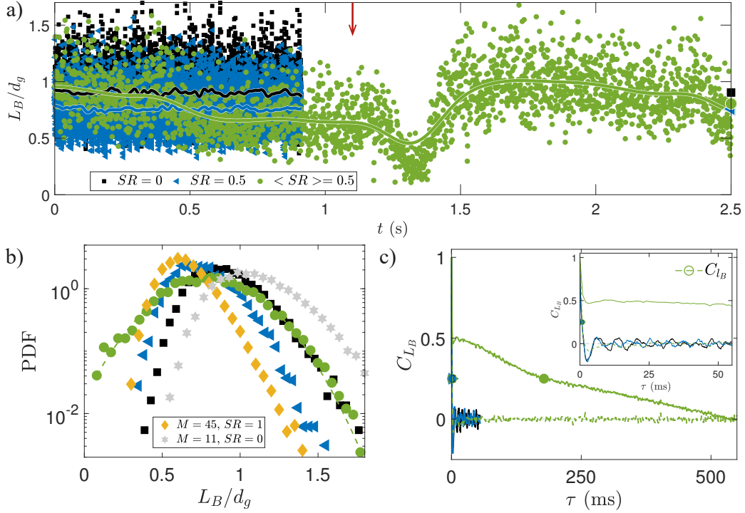
Figure 10: (color online) a) Time series of the liquid core length L_B normalized by the gas nozzle inner diameter d_g for M = 25 and SR = 0 (■), M = 25 and SR = 0.5 (◄) and \langle M \rangle = 25 and \langle SR \rangle = 0.5 (●). The thick lines show a moving mean and the corresponding symbols on the right vertical axis correspond to the time-averaged values over the whole series (only about a fourth of the time series is shown for the oscillating swirl condition that is recorded at a tenth of the frame rate but over 10 times the duration of the non-oscillating conditions). The red arrow indicates the time for the crest of one oscillation (local maximum of swirl and momentum ratio). b) Corresponding PDFs over the whole series, the dashed line is a Gaussian distribution defined by the mean and standard deviation of the liquid core length for the oscillating swirl condition. The PDFs for steady cases at the crest ( M = 45 and SR = 1 ♦) and trough ( M = 11 and SR = 0 ★) of the oscillation are added for comparison. c) Corresponding auto-correlation functions using the whole series. The additional green dashed lined represents the function calculated over the liquid core length subtracted by its moving average: l_B = L_B - \overline{L_B}(t)^T with T = 50 ms, for the oscillating swirl case. In the latter case, the functions cross the 0.25 threshold at 178.1 ms for L_B and 0.85 ms for l_B .
