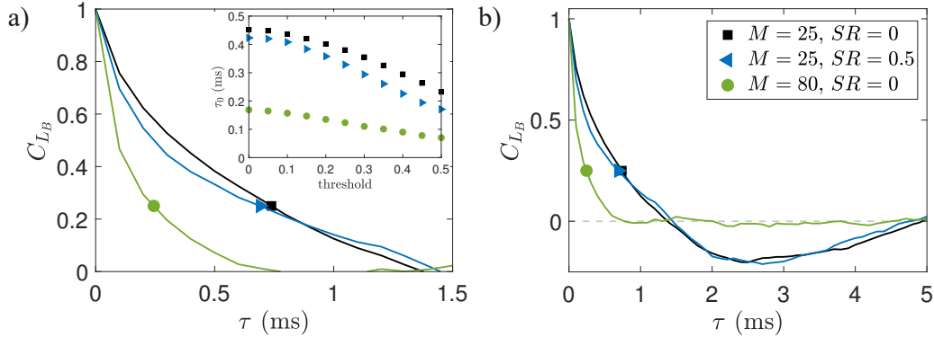
Figure 4: (color online) Auto-correlation of the liquid core length L_B over a narrow (a) and wider (b) range of time-lags \tau . The symbols (■, ◀, ●) show the times at which the functions reach a threshold of 0.25, respectively at 0.74, 0.69 and 0.24 ms for ( M = 25 , SR = 0 ); ( M = 25 , SR = 0.5 ) and ( M = 80 , SR = 0 ). The inset of (a) represents the liquid core length timescale \tau_0 , computed as the integral of the auto-correlation function up to the time at which it reaches a threshold value (varied between 0 to 0.5).
