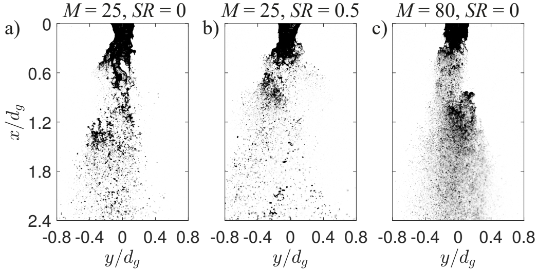
Figure 3: Back-lit images of the spray for a) ( M = 25 , SR = 0 ), b) ( M = 25 , SR = 0.5 ) and c) ( M = 80 , SR = 0 ). The images were background-corrected and the grayscale goes from 0 to 1.
