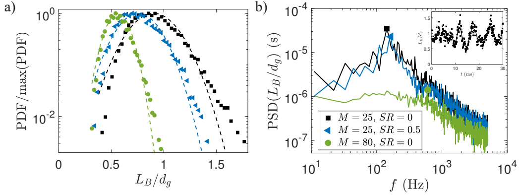
Figure 2: (color online) a) Probability density function (PDF) of the liquid core length L_B normalized by the gas nozzle diameter d_g ; the PDFs are normalized by their maximum value for clarity. The dashed lines correspond to Gaussian distributions defined by the mean and standard deviation of the liquid core length for each condition. b) Power spectral density (PSD) of L_B/d_g . The time series of L_B is cut in 10 pieces, each yield a PSD that are then averaged together to increase the signal-to-noise ratio in the frequency range of interest. The inset shows a small portion of the typical time-series of the liquid core length for ( M = 25 , SR = 0 ). The symbols ( \blacksquare , \blacktriangleleft , \bullet ) show the locations of the maxima of the PSDs, respectively at 142.9; 164.8 and 604.4 Hz (with a resolution of 11 Hz) for ( M = 25 , SR = 0 ); ( M = 25 , SR = 0.5 ) and ( M = 80 , SR = 0 ).
