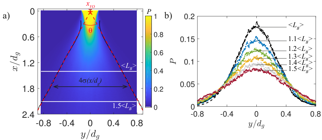
Figure 5: (color online) a) Probability of liquid presence (inferred from the back-lit images, through background subtraction, renormalization and thresholding, followed by ensemble averaging). b) Transverse profiles of the probability of liquid presence, for various longitudinal distances from the nozzle exit plane, \langle L_B \rangle \leq x \leq 1.5 \langle L_B \rangle ; they are fitted well by Gaussian distributions, A \exp(-(y/d_g)^2/2\sigma^2) , where A and \sigma are functions of x . The values of \pm 2\sigma(x) are reported on (a) by black dots when the Gaussian fits have R^2 values larger than 0.99, over the range of measured longitudinal distances, shown every 0.025 d_g for visibility. The function 2\sigma(x/d_g) is fitted linearly, between \langle L_B \rangle and 1.5 \langle L_B \rangle depicted as white lines here, to measure the spray angle \theta and virtual origin x_{VO} (where the two red dotted lines cross). The condition for a) and b) is M = 5 and SR = 0 .
