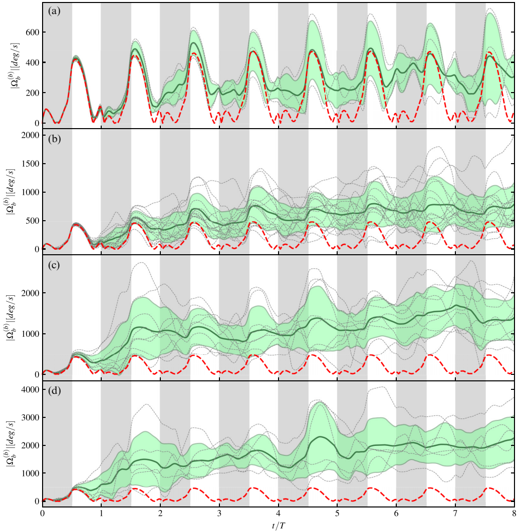
FIG. 9. Free flight in turbulent inflow, I = 0.16 (a), 0.33 (b), 0.60 (c), and 0.99 (d), for fixed \Lambda = 0.77 . Time evolution for the magnitude of body angular velocity. Individual realizations are shown as thin, gray, dashed lines. Ensemble averaged time evolution is represented by the thick green line and the light green shaded background illustrates the standard deviation. The red dashed line corresponds to the laminar case.
