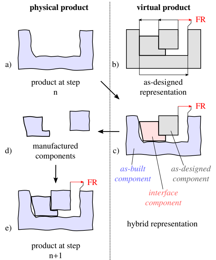
Figure 2: The proposed hybrid virtual representation (c) is created from the initial as-designed representation of the product (DMU) (b) and the physical product (a) so that the extracted manufacturing and assembly operations (d) result in a final product which fulfills its functional requirements (FR) (e).
