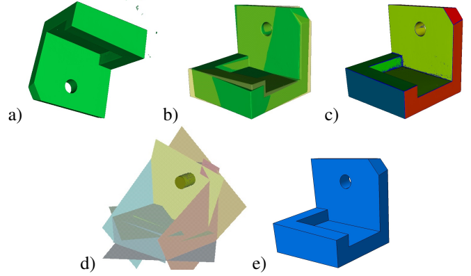
Figure 17: (a) acquired mesh, (b) registered mesh (as-designed component in transparent yellow), (c) classified mesh, (d) fitted surfaces, (e) as-built CAD component.
