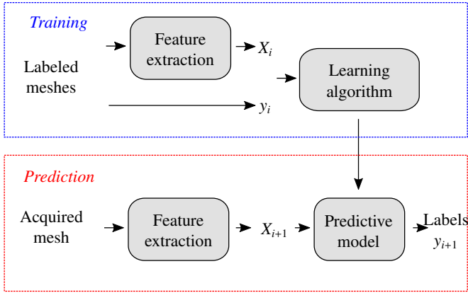
Figure 7: Supervised classification framework.
