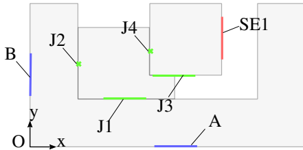
Figure 6: Example of geometrical skeleton.
