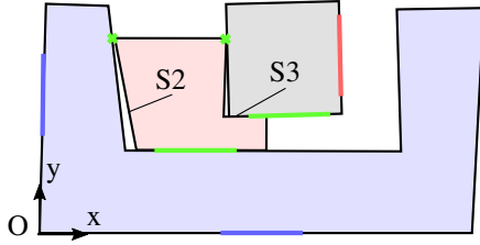
Figure 9: Update of the interface component.
