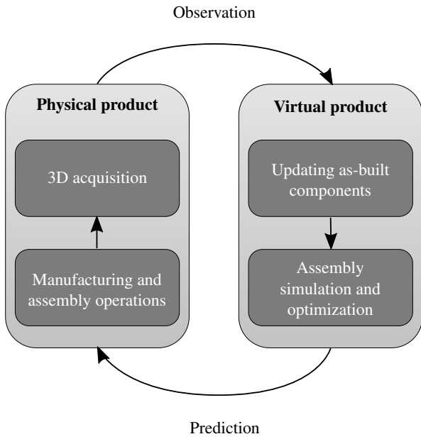
Figure 1: Digital twin based approach for the management of geometrical deviations during assembly.
