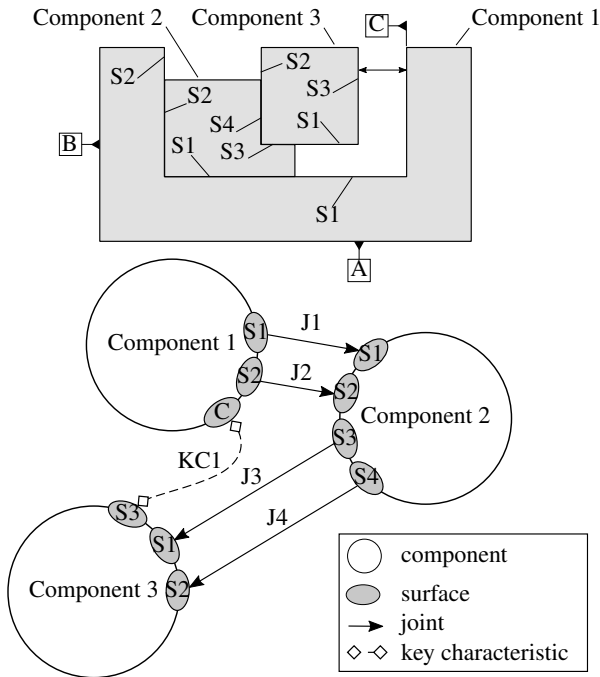
Figure 4: Example of Oriented Contact Graph.
