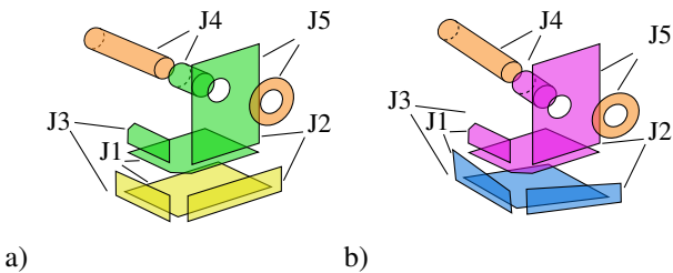
Figure 14: Surfaces defining the assembly joints (a) initial product representation (b) hybrid product representation.
