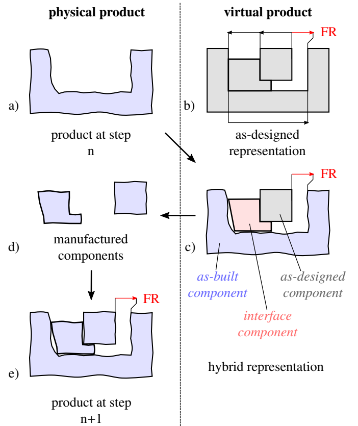
Figure 2: The proposed hybrid virtual representation (c) is created from the initial as-designed representation of the product (DMU) (b) and the physical product (a) so that the extracted manufacturing and assembly operations (d) result in a final product which fulfills its functional requirements (FR) (e).
