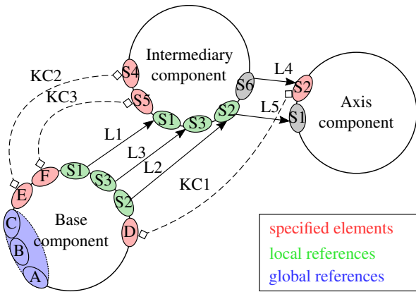
Figure 13: Oriented Contact Graph of our case study product.
