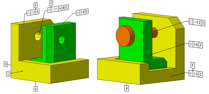
Figure 10: Initial product DMU showing the partial representation for our case study functional requirements.
