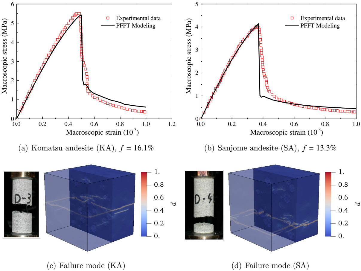
Figure 30: Comparisons between the experimental data from Hashiba and Fukui (2015) and the PFFT modeling results under uniaxial tension test
