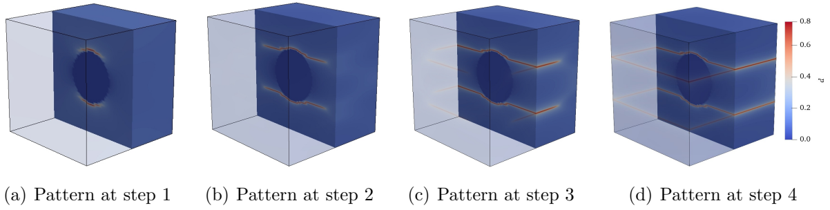
Figure 19: Crack patterns of the unit cell under uniaxial tensile test: \eta = 10^4 Pa.s
