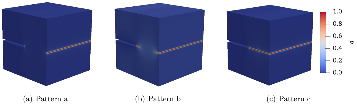
Figure 6: Crack growth patterns visualized by red color of a single notched unit cell under uniaxial tensile test
