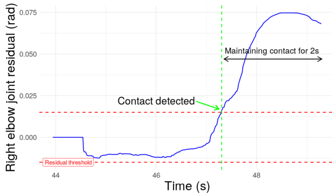
Fig. 9: Right end-effector contact detection
