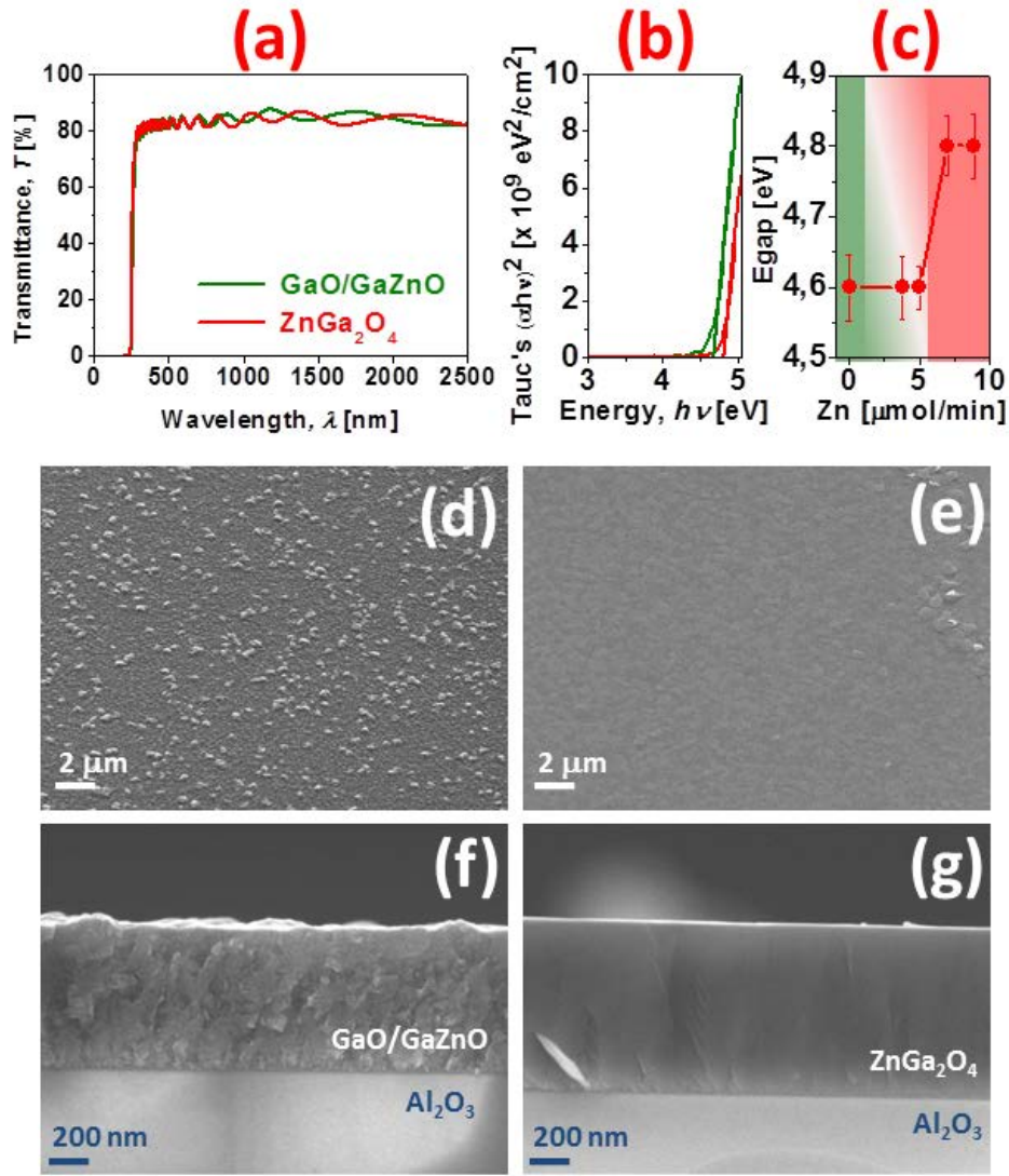
Figure 2. (a) Optical transmittance. (b) Tauc's plots (for the determination of the optical bandgap energy) for GaO/GaZnO mixed phase and for the pure ZnGa 2 O 4 . (c) Optical bandgap energy versus Zn-flux ( \mu\text{mol/min} ) used during the growth. (d) and (e) top view SEM images of the GaO/GaZnO mixed phase and the pure ZnGa 2 O 4 . (f) and (g) cross sectional SEM images of the GaO/GaZnO mixed phase and the pure ZnGa 2 O 4 .
