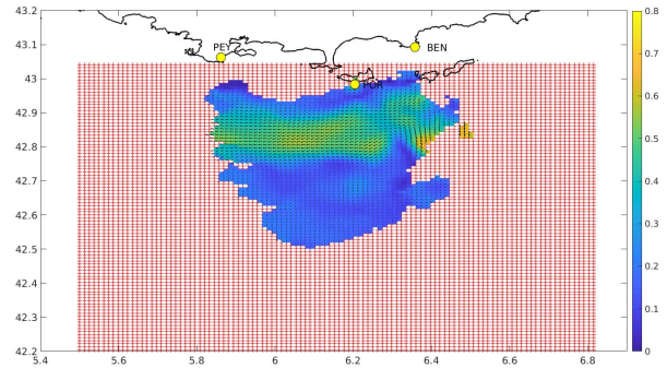
Fig. 7. Recombined elliptical radials of the surface current for a one hour observation on February 4, 2019 (14:00-15:00 UTC). Only the area with 4 simultaneous existing radials are reconstructed. The colorscale is in m/s.
