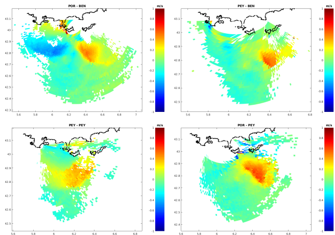
Fig. 5. Four simultaneous elliptical radials maps resulting from a 1 hour observation time on February 4, 2019 (14:00-15:00 UTC).
