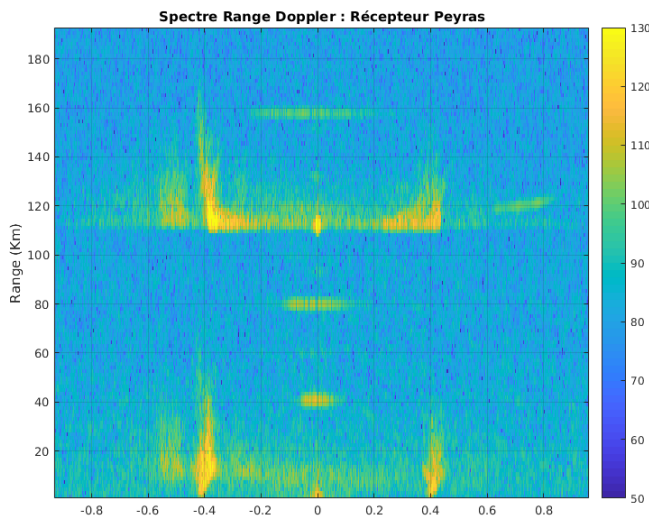
Fig. 4. A multistatic range-Doppler map seen from Fort Peyras
