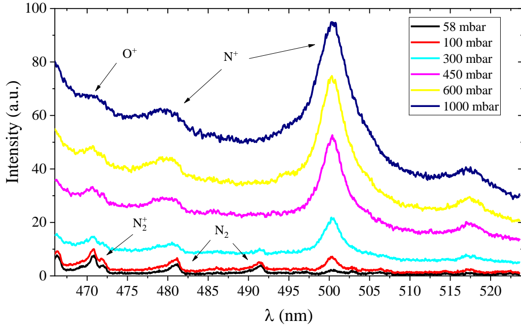
Figure 6 Measured emission spectra (middle of the gap) integrated from t = 0 to 10 \text{ ns} at several pressures. The interelectrode gap is 0.9 \text{ mm} (setup #1). For the sake of clarity, only six spectra are displayed.
