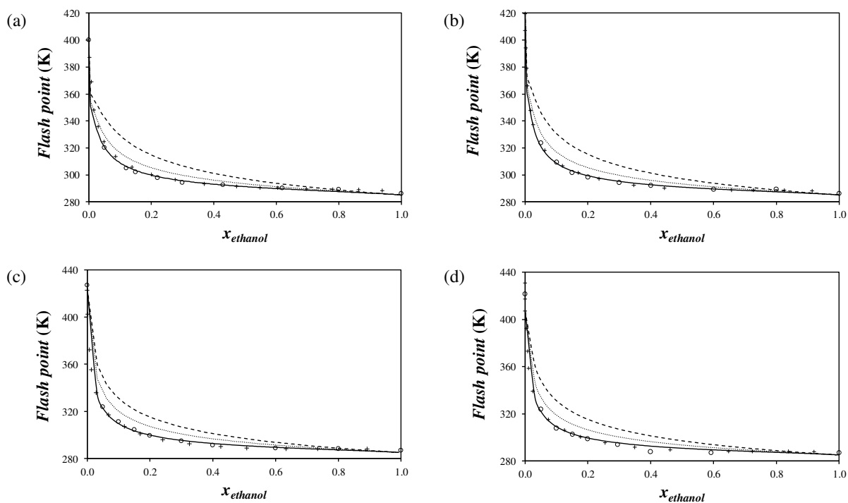
Figure 2. Flash points of ethanol + ethyl ester mixtures (a) ethanol + ethyl laurate (dodecanoate), (b) ethanol + ethyl myristate (tetradecanoate), (c) ethanol + ethyl oleate (technical grade), (d) ethanol + ethyl biodiesel made from palm oil. The compositions of the palm oil biodiesel and technical grade ethyl oleate are provided in the supplementary materials (Table A6). Comparison between experimental data [22] (circles) and the Catoire-Naudet model combined with Raoult's law (dashed curves), COSMO-SAC (dotted curves) and COSMO-SAC dsp (solid curves). The pluses (+) correspond to the model of Carareto et al. [22].
