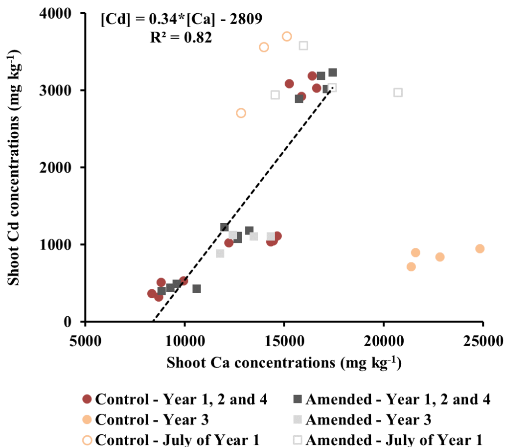
Fig. S23: Relationship between Cd and Ca concentrations in the shoots of N. caerulea . A linear regression was used on the data from both lysimeters at October's harvest of Year 1, Year 2 and Year 4. Data from Year 3 and from July of Year 1 is also indicated on the graph, but was not taken into account in the linear regression.
