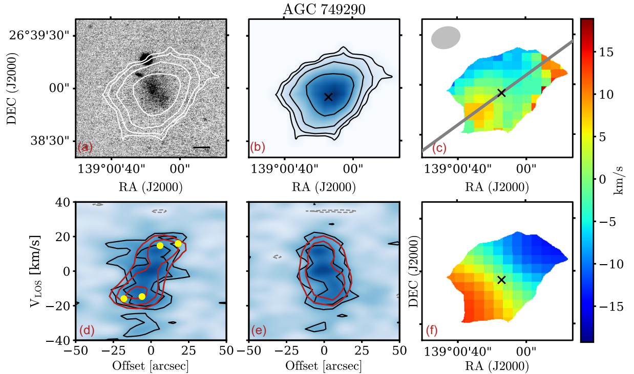
Figure 6. Data and kinematic models for the gas-rich UDG AGC 749290. Panels and symbols as in Fig. 1. The H I contours are at 0.35, 0.7, 1.4, and 2.8 \times 10^{20} atoms \text{cm}^{-2} . As shown in the major-axis PV diagram (panel d), while {}^3\text{D}_{\text{BAROLO}} models well the main rotating body, there is signal at around velocities of 10 \text{ km s}^{-1} and offset 25 \text{ arcsec} that cannot be reproduced by the best-fitting model. The parameters for these galaxy are considered less robust than for the rest of the sample, as we discuss in Section 3.2.
