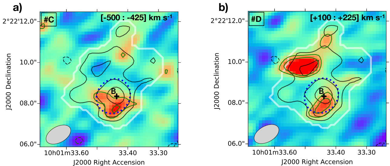
Fig. B.1. (a) Velocity-integrated [CII] maps of #C and (b) #D, obtained by collapsing the spectral channels corresponding to a 2 \times \text{FWHM} interval centred on their z_{\text{[CII]}} (see spectra in Fig. 4a, and values in Table 1). The velocity ranges used to collapse the datacubes are shown in the top-left corners. The rest-frame UV centroid of #B is indicated with a plus symbol. The dashed blue ellipse defined in Fig. 3 (see Sec. 3.3) is shown for reference. The grey solid line and the black contours indicate the significance level of the [CII] flux emitted by the full system as defined in Fig. 4b. The green solid (dashed) contours indicate the positive (negative) significance levels at [3,4]\sigma of the [CII] flux maps of #C (a) and #D (b). To help the visualization of (b), we used a maximum value of surface brightness in the colour-map range as defined by excluding the bright spot at North (corresponding to a fraction of the emission of #A). The ALMA beam size is given in the bottom-left corner. North is up and east is to the left.
