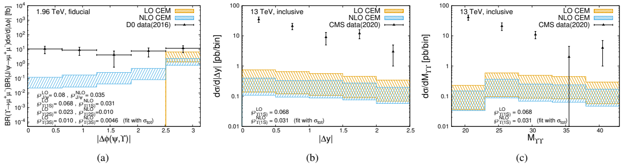
Figure 3: Comparison between our LO and NLO CEM computations and the experimental data for (a) the |\Delta\phi| distribution of J/\psi + \Upsilon at the Tevatron and (b) the |\Delta y| & (c) M_{\Upsilon\Upsilon} distributions of di- \Upsilon at the LHC.
