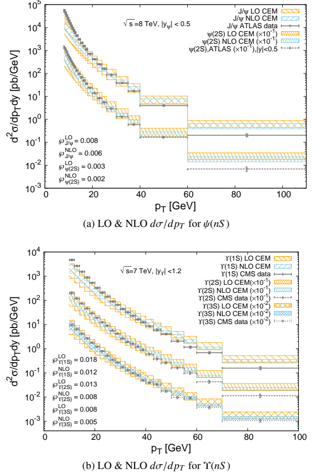
Figure 1: The p_T (and y ) differential cross sections of single (a) J/\psi and \psi(2S) and (b) \Upsilon(nS) ( n = 1, 2, 3 ) production in the CEM. The plotted data from ATLAS (8 TeV) [75] and from CMS (7 TeV) [76] were used to fit \mathcal{P}_Q^{(\text{N})\text{LO}} .
