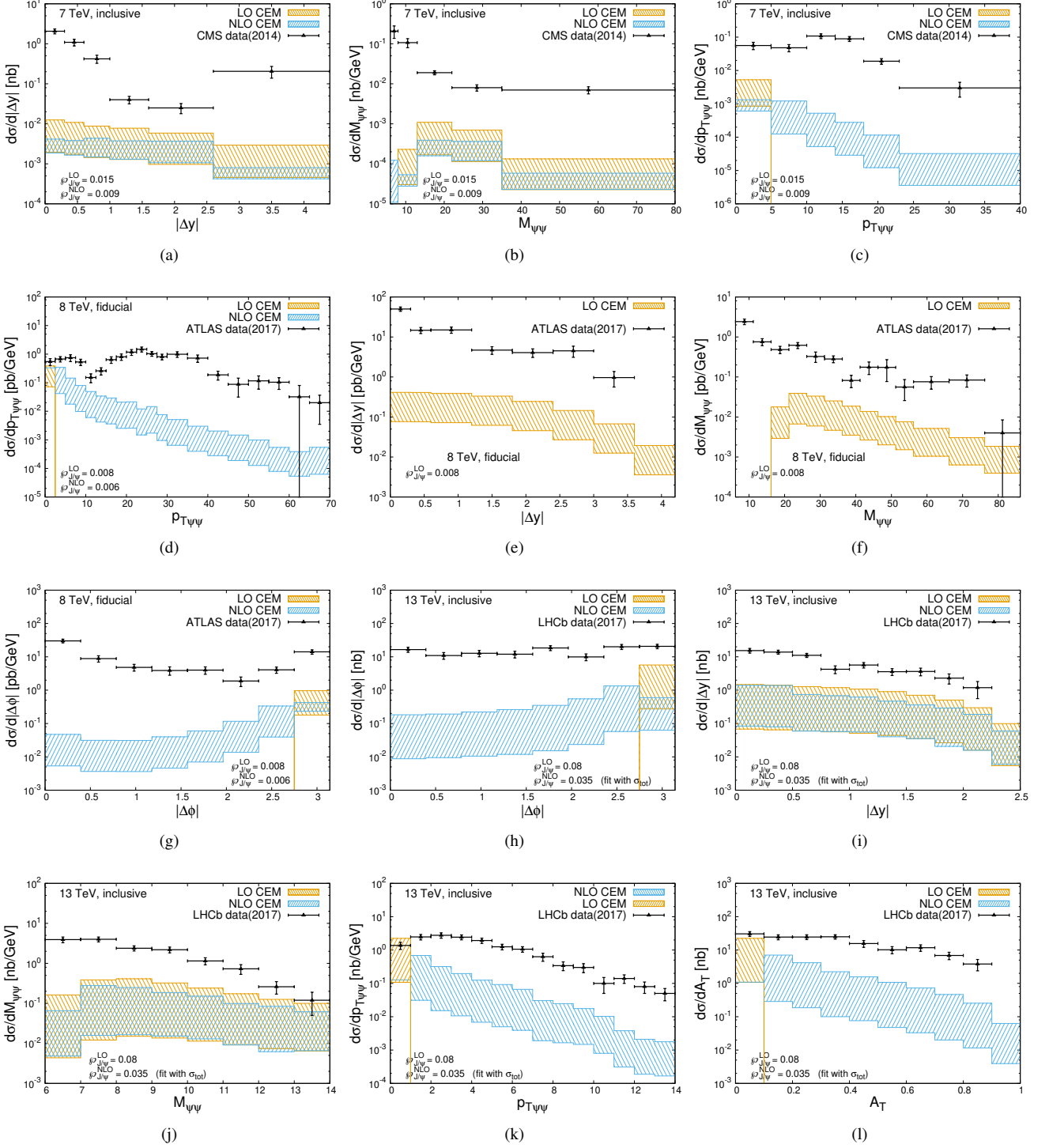
Figure 2: Various existing kinematical distributions of di- J/\psi events compared to our LO and NLO CEM computations. See text for details.
