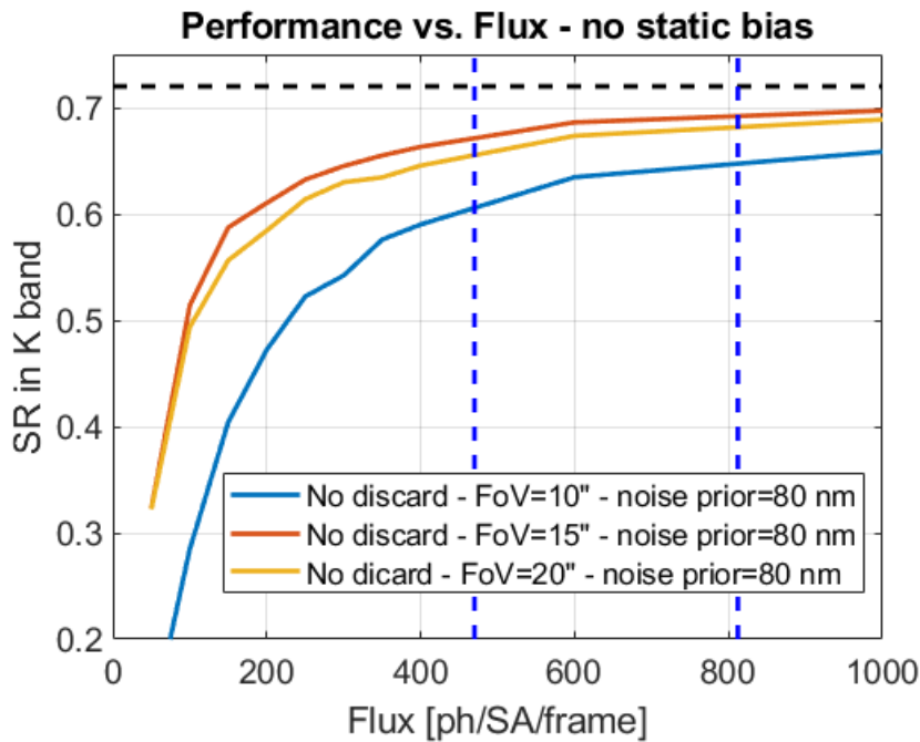
Figure 9: On axis performance as a function of flux - no eigen vector is discarded - FoV=10" (blue) FoV=15" (red) FoV=20" (yellow) Reference with no elongation (dash black) Flux level at 90 th and 50 th percentile (dash blue)
