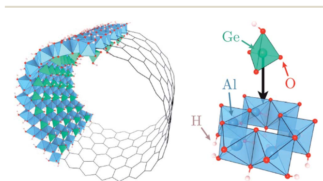
Fig. 1 Polyhedral representation of a SW Ge-INT where O 3 Al(OH) 3 octahedra (in blue) are arranged to form a honeycomb network and O 3 GeOH tetrahedra (in green) are placed right above each octahedral cavity.
