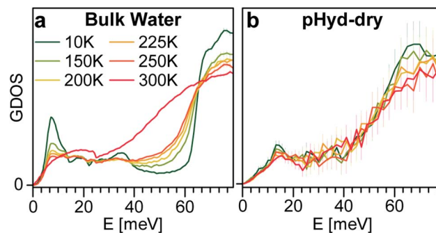
Fig. 4 Generalised density of state (GDOS) as a function of temperature: (a) bulk water and (b) GDOS of pHyd nanotubes minus GDOS of dry nanotubes.
