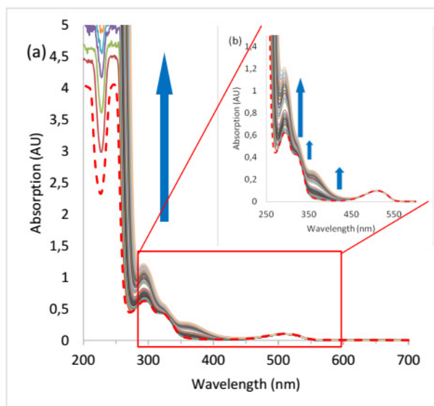
Figure 5. Absorption spectra measured during the titration of 1 with tetrabutylammonium chloride (from 0 to 70 equivalents of TBACl): a) total spectrum b) zoom
