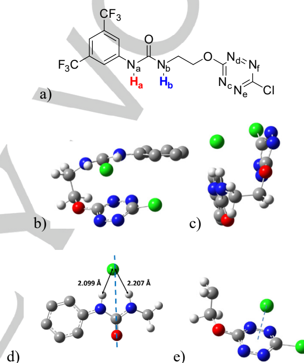
Figure 1. a) Labelling system and selected views of 1-Cl (CF 3 groups are omitted for clarity). b) and c) front and side views of cofacial arrangement between the urea/Cl - and the tetrazine planes. d) position of Cl - with respect to median axis of the urea. e) distance between Cl - and the tetrazine centroid.
