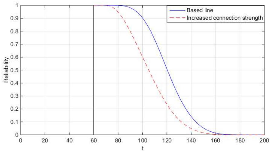
Fig. 11. Sensitivity analysis of connection strength on the system reliability
