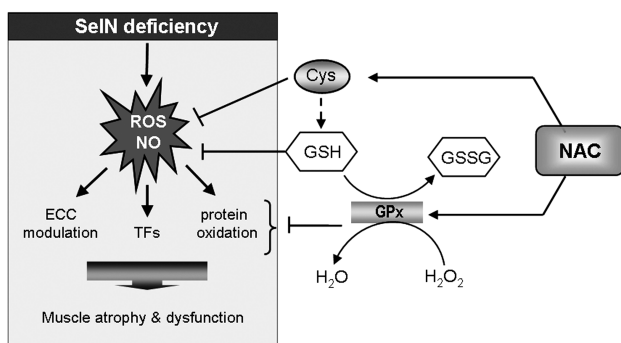
FIG. 4. Mechanisms of action and pathophysiological targets of N-acetyl cysteine (NAC) in SEP1N-related myopathy. ECC: excitation-contraction coupling; GPx: glutathione peroxidase; TFs: transcription factors.
