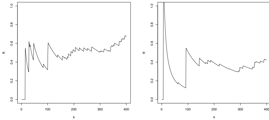
Figure 10: Vehicle insurance dataset. \widehat{R}(2, 2|x_0) as a function of k , for x_0 = 35000 (left) and x_0 = 85000 (right).
