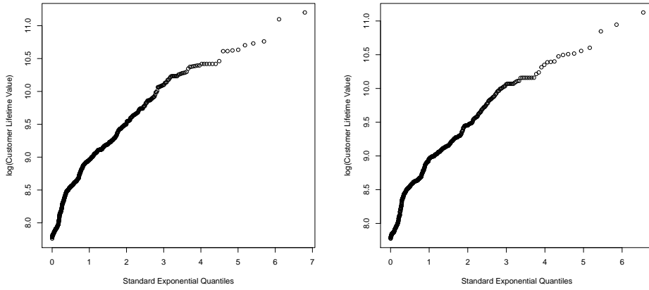
Figure 9: Vehicle insurance dataset. Pareto quantile plots of the customer lifetime value for which income \in [30000, 40000] (left) and income \in [70000, 80000] (right).
