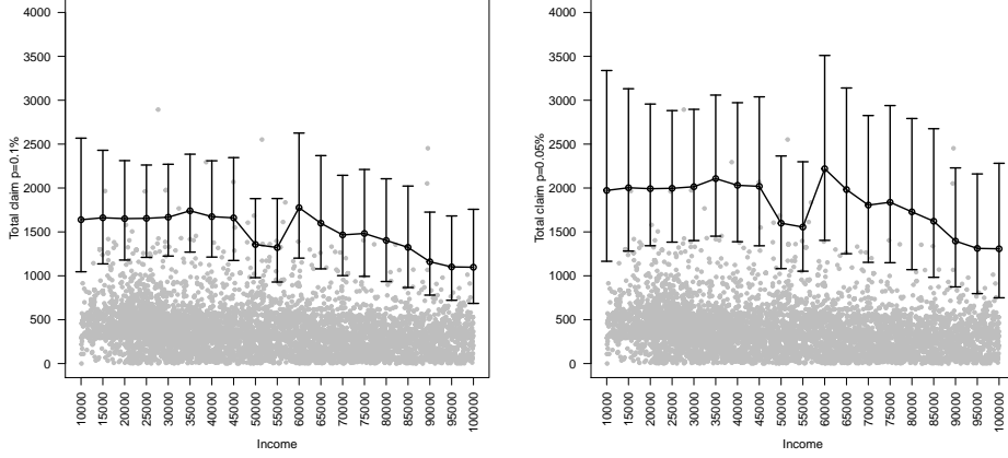
Figure 11: Vehicle insurance dataset. \hat{\theta}_p(x_0) along with pointwise 95% confidence intervals for \theta_p(x_0) at several values of x_0 for p = 0.1\% (left), p = 0.05\% (right).
