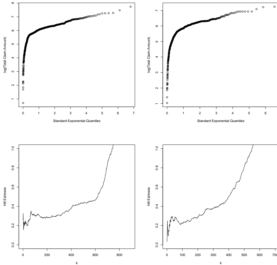
Figure 8: Vehicle insurance dataset. Top row: Pareto quantile plots of the total claim amount for which income \in [30000, 40000] (left) and income \in [70000, 80000] (right). Bottom row: Hill estimates of the total claim amount for which income \in [30000, 40000] (left) and income \in [70000, 80000] (right).
