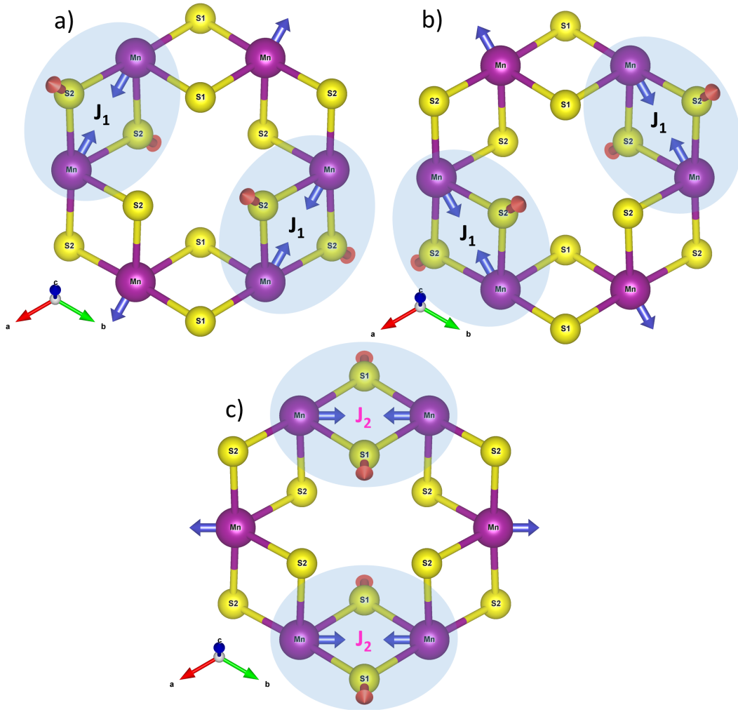
FIG. S4. Virtual atom displacements that would change the corresponding superexchange angles associated to the effective exchange interactions. Phonon mode visualizations were drawn with VESTA [1].
