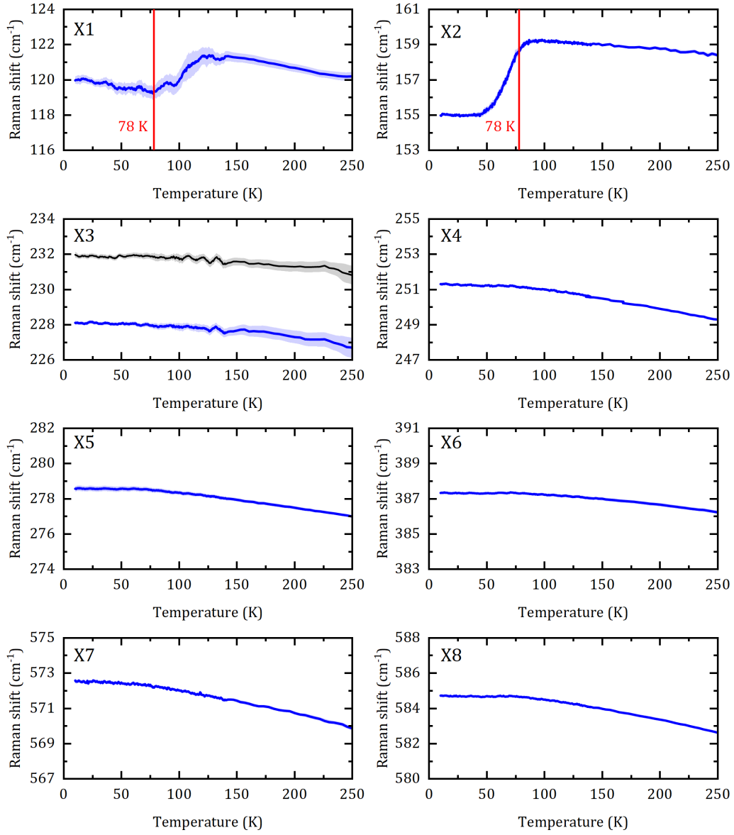
FIG. S1. Temperature dependence of the central positions of phonon-related, X1, .. X8, Raman scattering lines in \text{MnPS}_3 .
