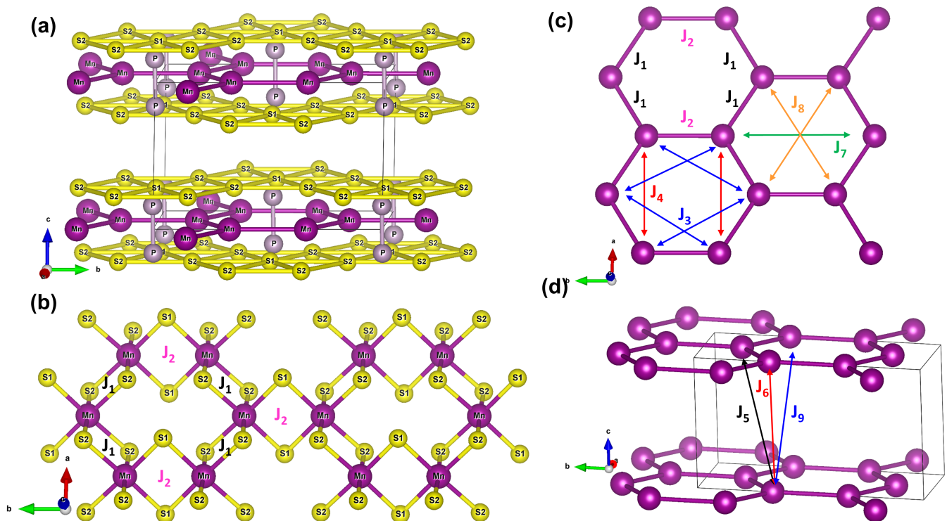
FIG. 1. (a) Atomic structure of MnPS 3 . Mn atoms are represented in violet, S in yellow, and P in gray. (b) Detail of the Mn - S bonds in the Mn-S-Mn sandwiches. The S 1 sulfur atoms are associated to the super-exchange path that controls the effective magnetic interaction J 2 . Similarly the S 2 sulfur atoms are associated to the effective magnetic interaction J 1 . (c) Detail of the six intralayer effective exchange interactions considered in this work. The difference between J 1 and J 2 , J 3 and J 4 , and J 7 and J 8 is a consequence of the distortion of the honeycomb lattice. (d) Detail of the three interlayer effective exchange interactions considered in this work. Atomic structures were drawn with VESTA [5].
