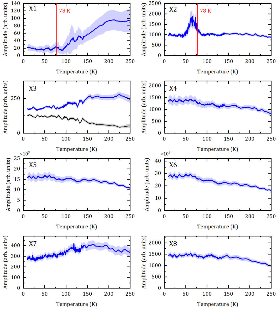
FIG. S3. Temperature evolution of the amplitude of phonon-related, X1, ..X8, Raman scattering lines in MnPS 3 crystals.
