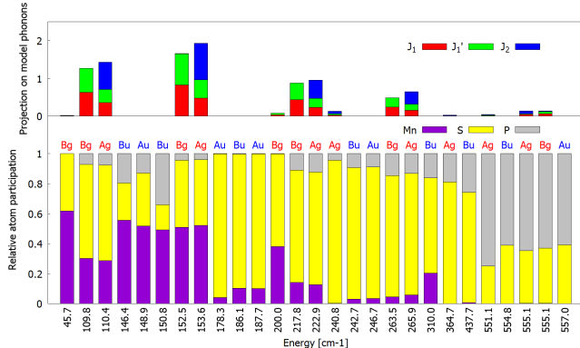
FIG. 6. Upper panel: projection of the optical phonon modes in the three virtual modes shown in Fig. S4 in Supplementary Material. Lower panel: relative atomic participation in the optical phonon modes of MnPS 3 of the three atom's types. The colors in the bars represent the contribution of the two Mn atoms (violet), the six S (yellow), and the two P atoms (gray). The symmetry of the modes is shown in the upper part of the figure.
