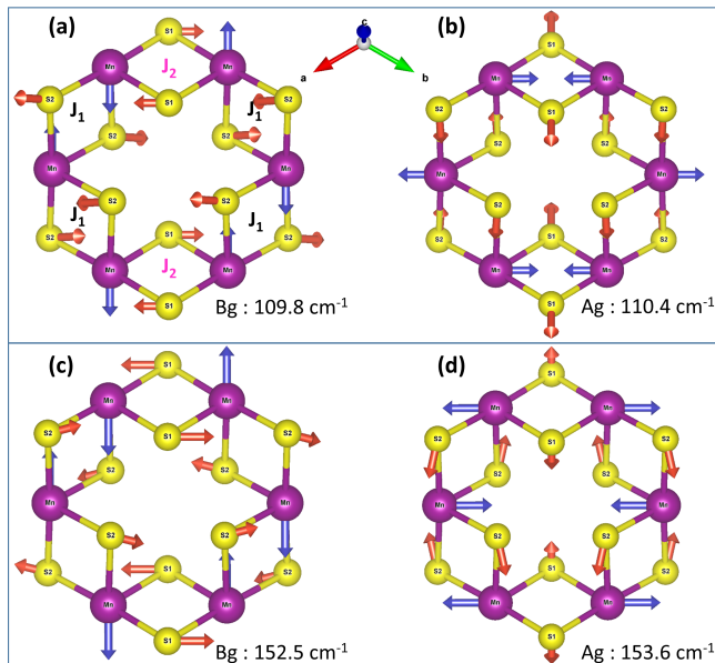
FIG. 7. Schematic representation of the displacements of the Mn and S atoms in \text{MnPS}_3 corresponding to the two pairs of Raman active modes associated to the experimental peaks X1 and X2. Phonon mode visualizations were drawn with VESTA [5].
