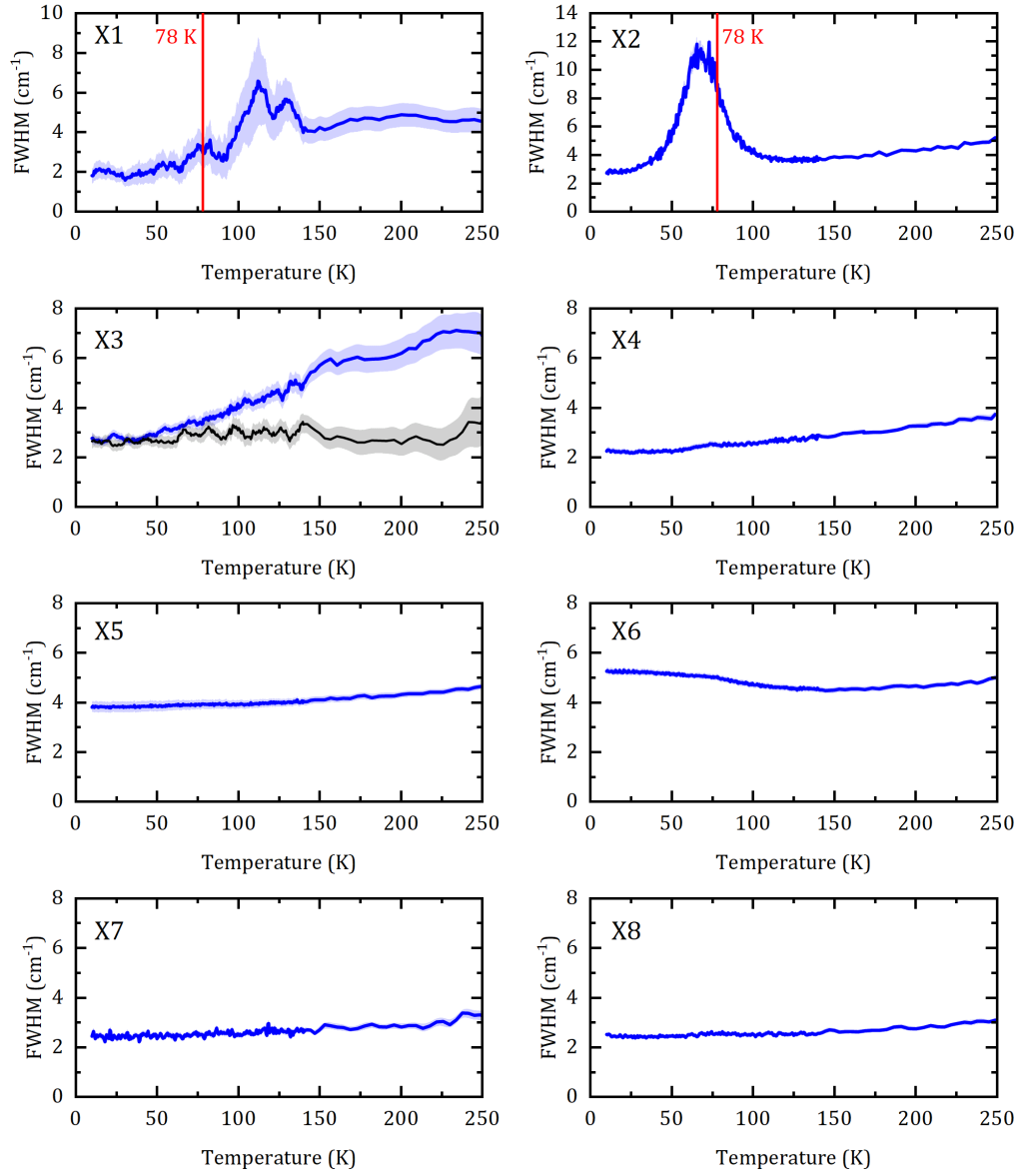
FIG. S2. Evolution with temperature of the full width at half maximum FWHM of phonon-related, X1, ...X8, Raman scattering lines in \text{MnPS}_3 crystals.
