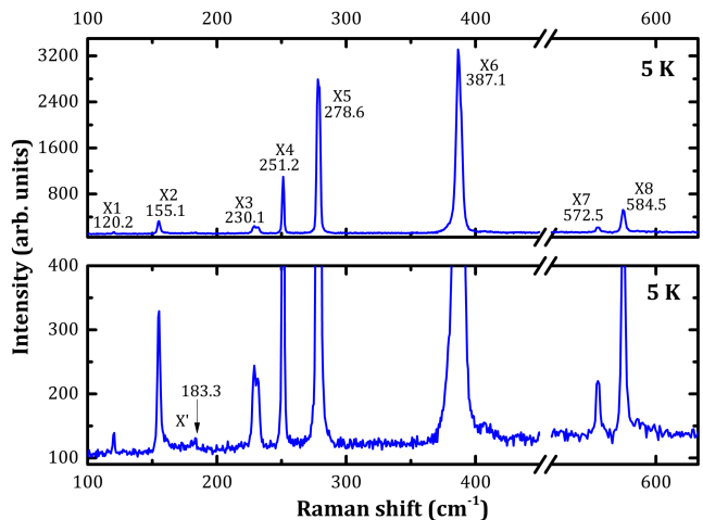
FIG. 2. Characteristic Raman scattering spectrum of the MnPS 3 crystal, measured under 514 nm laser line excitation, at low temperature ( T = 5 K) in a wide spectral range 100 to 650 \text{cm}^{-1} from the laser line. The spectrum shown in the upper (a) panel is expanded in vertical direction in the bottom (b) panel to better visualize the less intense Raman-scattering modes. The observed narrow X1 ... X8 Raman scattering peaks are due to phonons whereas a broad X' feature with the high energy onset at 183.3 \text{cm}^{-1} is of different origin.
