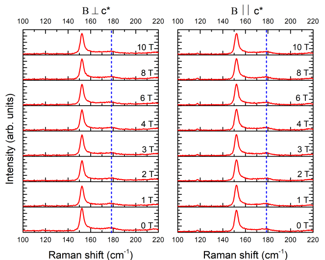
FIG. 4. Evolution of the X2 and X' peaks with an applied magnetic field oriented perpendicular (left) and parallel (right) to the reciprocal lattice vector c^* . The experiment was performed at 5 K.
