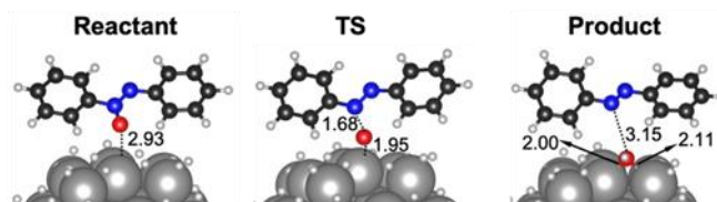
Fig. 8 Optimized structures for azoxynitrobenzene intermediate adsorbed on H 88 Ru 57 nanoparticle, the diphenylhydrazine resulting from its hydrogenation and the transition state connecting them. Distances in Å and energies in kcal mol -1
