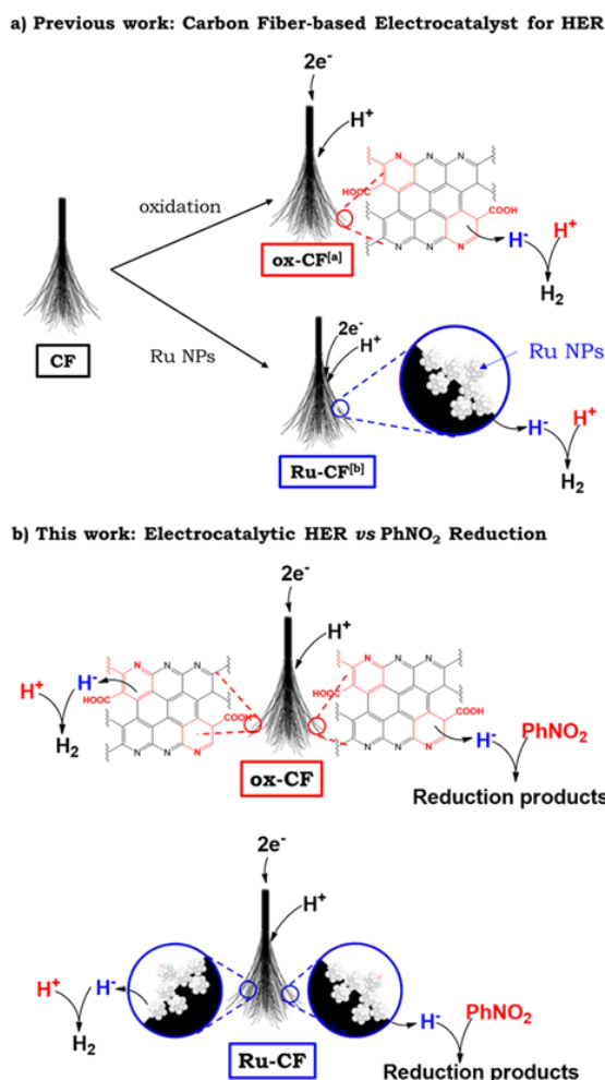
Fig. 1 Schematic representation of a) Carbon Fibre-based electrocatalysts for HER (previous work) 21,27 and b) HER vs hydrogenation of PhNO 2 using same electrocatalysts (this work).
