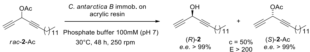
Fig. 3. Lipase-mediated kinetic resolution of rac-2 -Ac without a co-solvent.
