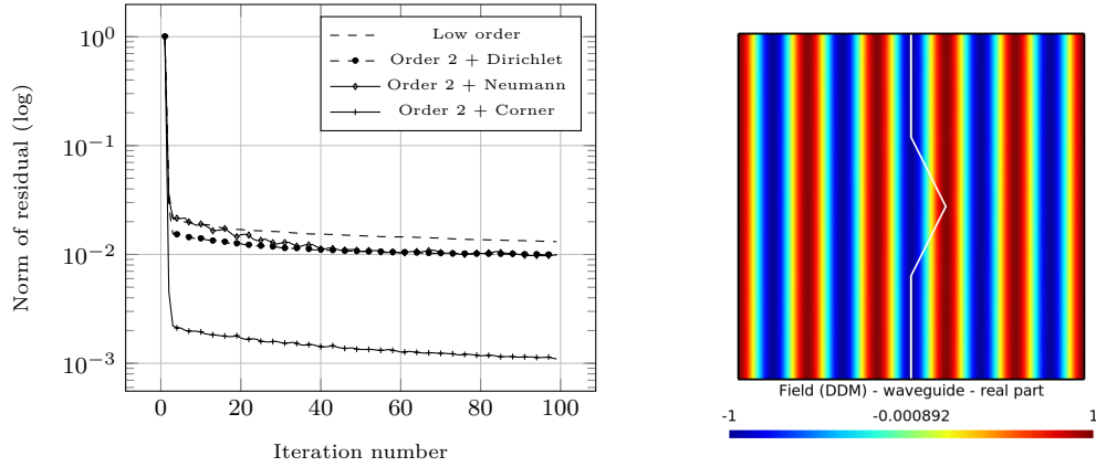
Fig. 10: Waveguide problem. Robin conditions are set on the left and on the right of the square: heterogeneous with a plane wave as a source on the left ( -\partial_x u - \mathbf{i}\omega u = e^{i\omega x} , with \omega = \pi ), homogeneous on the right ( \partial_x u - \mathbf{i}\omega u = 0 ). Two homogeneous Neumann ( \partial_{\mathbf{n}} u = 0 ) conditions on top and bottom of the domain. Left are shown the history of convergence of the Jacobi residuals for low order TC and 2 nd order TC with Dirichlet, homogeneous Neumann and the new corner conditions developed in this work. Right are displayed the solutions at (quasi-)convergence for the DDM with new TC. More details can be found on paragraph 5.4.1.
