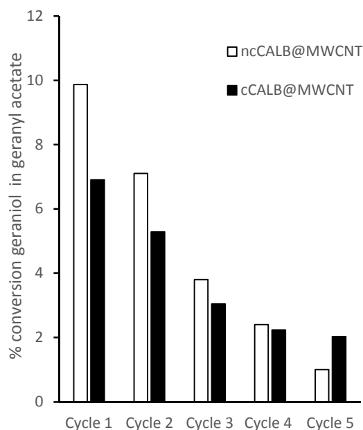
Figure 10 Conversion rate (%) of geraniol and acetate in geranyl acetate in scCO_2 using ncCALB@MWCNT (white bars) or cCALB@MWCNT (black bars). Experimental conditions: scCO_2 at 55°C and 200 bars, scCO_2 flow rate of 3.94 mL/min (3mL/min in liquid form), substrates concentrations of 43.4 mM in scCO_2 , approx. residence time in the fully charged 1 mL PBR was only 6 seconds, 132 mg of ncCALB@MWCNT or cCALB@MWCNT in the reactor, 300 mg of Lipozyme 435 beads, 30 min per run.
