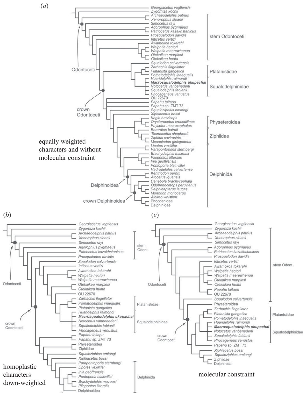
Figure 17. Alternative phylogenetic analyses using a modified matrix of Tanaka & Fordyce [6] and Lambert et al. [20]. (a) Strict consensus tree for the analysis with equally weighted characters and without molecular constraint; (b) strict consensus tree for the analysis with down-weighted homoplastic characters and without molecular constraint; (c) strict consensus tree for the analysis with equally weighted homoplastic characters and with molecular constraint (same result with down-weighted homoplastic characters). Note that in all of these analyses: (1) Macroscqualodelphis is inside Squalodelphinidae; (2) Squalodelphinidae are a monophyletic group and (3) Platanistidae and Squalodelphinidae are sister groups. The relationships within some clades (e.g. Delphinoidea in tree (b) and Delphinidae in tree (c)) were not shown because they are not relevant to the position of Macroscqualodelphis .
