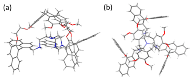
Figure 1. X-ray structure of P-(RRR)- 1 ·3H 3+ : (a) side view and (b) top view.
