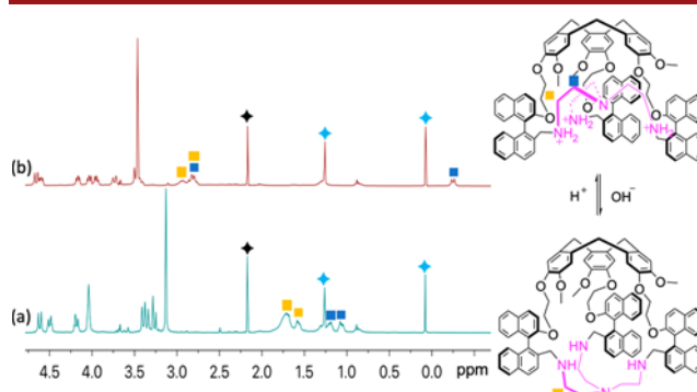
Figure 2. 1 H NMR (CDCl 3 , 400 MHz, 298 K) spectra of (a) P-(R,R,R)- 1 and (b) P-(R,R,R)- 1 ·3H 3+ . The black and blue ♦ represent acetone and grease, respectively.
