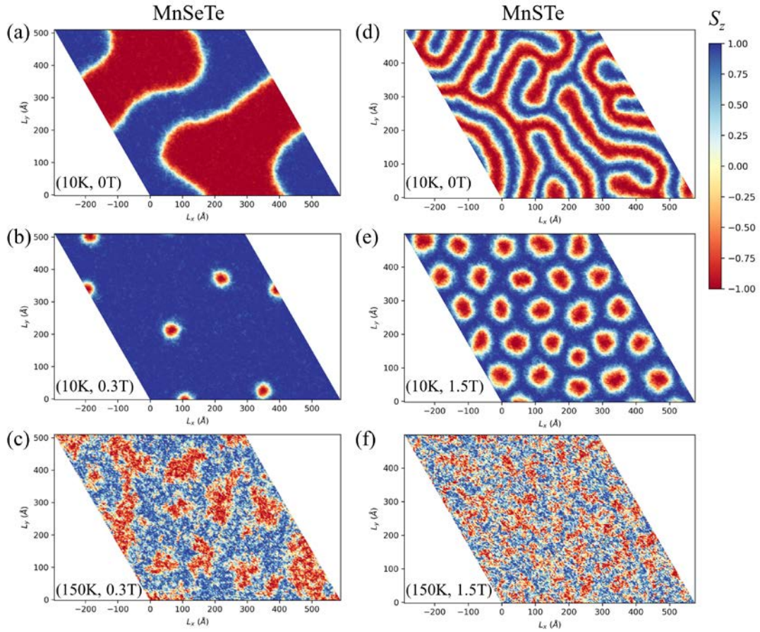
Figure 4. Spin textures for (a)-(c) MnSeTe and (d)-(f) MnSTe monolayers in real space. The corresponding temperatures and external fields for the simulations are labeled inside each figures. The color map indicates the out-of-plane spin component of Mn atoms.
