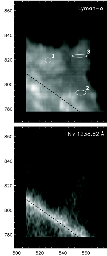
Fig. 4. SOHO/SUMER Lyman- \alpha and N v 1238.82 \text{ \AA} integrated intensity raster images obtained between 13:43 and 14:29 UT. Axes give the solar X and Y coordinates in arcsec. White ellipses indicate areas 1, 2, and 3.
