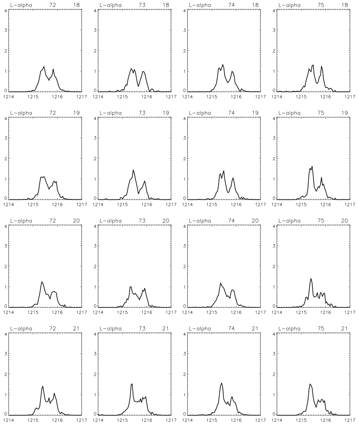
Fig. A.2. Small portion of the observed Lyman- \alpha profiles from AREA2. Numbers above each panel indicate the x and y positions in the SOHO/SUMER raster. The x -axis gives the wavelength in \text{\AA} , the y -axis the specific intensity in 10^{-8} \text{ erg s}^{-1} \text{ cm}^{-2} \text{ sr}^{-1} \text{ Hz}^{-1} .
