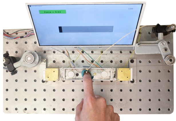
Fig. 3. Experimental setup. The subject touches the actuated glass plate on top of the force sensor. The finger is linked to a pulley-encoder system for position measurement and an accelerometer is placed on the first phalanx. The screen shows a cursor imposing the velocity and provides feedback on the normal force.
