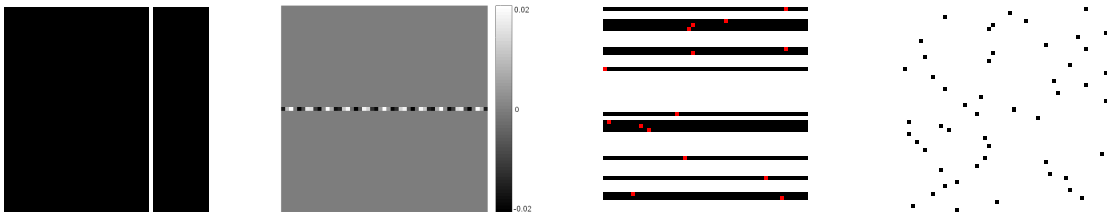
Figure 2: Example of a kernel associated with hard core repulsion in the horizontal direction. From left to right, the Fourier coefficients of C , the real part of the kernel C , a capture of the conditional density during the simulation, the associated final sample.
