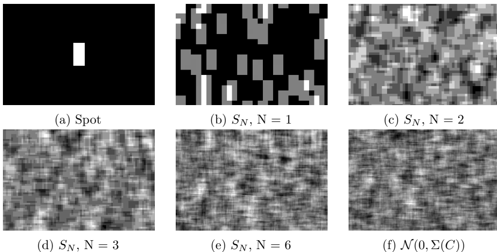
Figure 4: Determinantal shot noise realizations S_N as defined in Theorem 11 with various N = 1, 2, 3, 6 and a comparison with their associated limit Gaussian random field \mathcal{N}(0, \Sigma(C)) (f). The shot noise is based on the spot (a) and the projection DPixP with kernel C whose non-zero Fourier coefficients form a disk (Figure 1, bottom).
