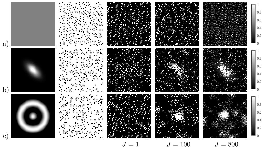
Figure 8: Experiments on general DPixP kernels. From left to right : the target Fourier coefficient of the kernel we want to recover, one realization of this DPixP, the estimation of the Fourier coefficients from one, from 100 and from 800 realizations, with k_{\max} = 2000 .
