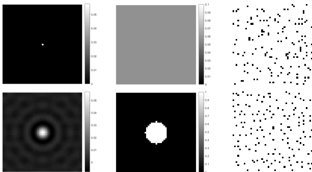
Figure 1: Comparison between two samples (both have 148 points) of a Bernoulli process (first line) and a projection DPixP defined by the kernel C such that \hat{C} is the indicator function of a discrete circle (second line). For both DPixPs, from left to right, the real part of the kernel function C , its Fourier coefficients \hat{C} and one associated sample.
