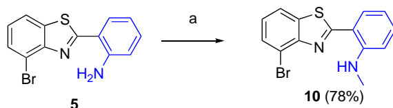
Scheme 3: Monomethylation of 5
