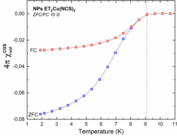
Fig 4. Temperature dependence (in blue) of the zero-field cooling (ZFC) and (in red) of the field cooling (FC) of the NPs. The dash line indicates T_c = 9.1K .
