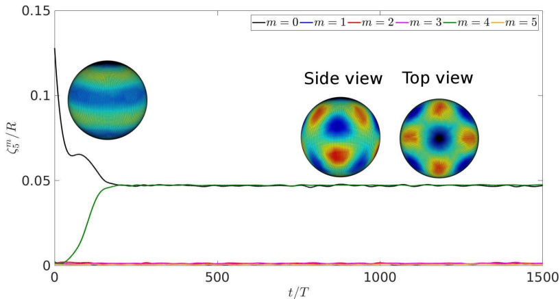
FIGURE 25. Timeseries of m components for an \ell = 5 pattern. An initially axisymmetric pattern with m = 0 briefly equilibrates and is then replaced by a D_4 pattern, which is a superposition of m = 0 and m = 4 .
