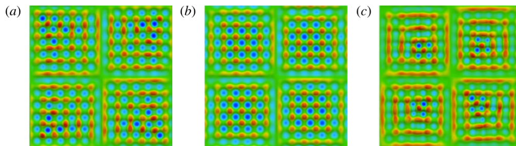
FIGURE 3. Snapshots of the top view of the interface colored by the vertical velocity for (a) no-slip, (b) free-slip, and (c) periodic boundary conditions.
