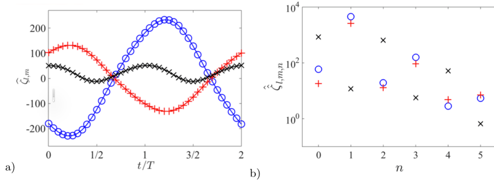
FIGURE 8. a) Temporal evolution of the three main spatial modes. Modes \hat{\zeta}_{23,1} (blue curve and circles) and \hat{\zeta}_{23,3} (red curve and + symbols) are subharmonic: their period of oscillation is twice that of the forcing. Mode \hat{\zeta}_{46,0} (black curve and \times symbols) is harmonic. b) Temporal spectrum of the main modes. \hat{\zeta}_{23,1} , \hat{\zeta}_{23,3} contain only odd temporal harmonics while \hat{\zeta}_{46,0} has mainly even harmonics. Each spatial mode has a finite n = 0 component and hence a non-zero temporal mean.
