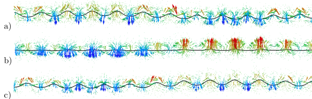
FIGURE 5. Velocity profiles on the plane y = 3L/4 , corresponding to each of the three instants shown in figure 4. The vectors are colored according to their vertical component.
