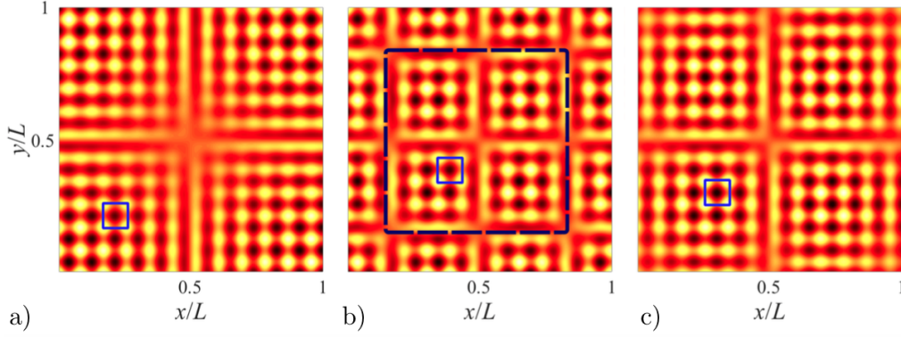
FIGURE 7. Patterns constructed from Fourier modes (a) in \mathcal{C}_1 , (b) in \mathcal{C}_3 , and (c) a superposition of the two. Lighter (darker) zones correspond to the peaks (troughs) of the interface. Superlattices, consisting of smaller and larger squares, are observed in all of the plots. Smallest boxes are approximately of size \lambda_c . b) Medium squares of size 2L/3 are present (long-dashed box). c) Reconstructed pattern, made by combining patterns in (a) and (b) weighted by the corresponding Fourier coefficients \hat{\zeta}_{23,1} and \hat{\zeta}_{23,3} . Compare with figure 4(c).
