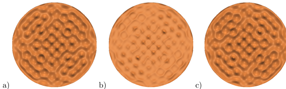
FIGURE 9. Interface profile in the cylinder at time intervals of T/2 . The central part of the domain is still occupied by squares, but five-sided cells are present near the boundaries, allowing the pattern to fit inside a circle.
