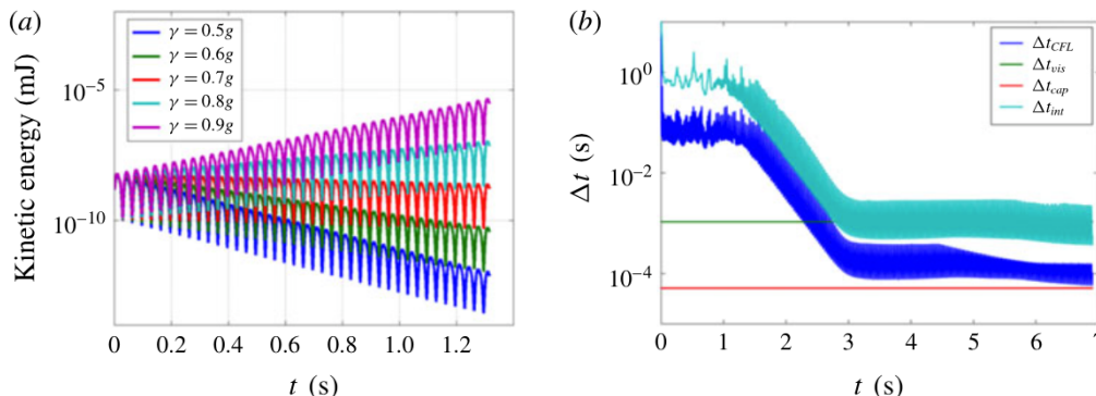
FIGURE 1. a) Evolution of the total kinetic energy for \omega/2\pi = 30 Hz and various accelerations in a small domain. The fact that the peaks for a given acceleration lie along a line shows that the energy growth is very close to exponential. b) Evolution of the various bounds on the time step during the course of the simulation. The smallest, \Delta t_{cap} , is used in the simulations.
