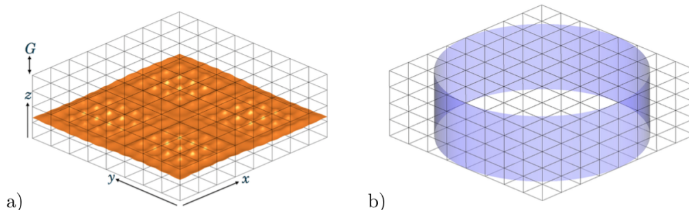
FIGURE 2. Calculation domain of size L \times L \times L/3 ( L = 132 mm), divided into 8 \times 8 \times 4 subdomains. a) Interface profile. b) an immersed solid cylinder of diameter D = L and height h = L/3 surrounding the flow. The flow outside of the cylinder is not computed. For both (a) and (b) the Cartesian resolution per subdomain is 64^3 , which gives a global resolution of 512 \times 512 \times 256 .
