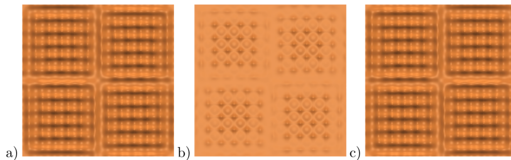
FIGURE 4. Interface profiles at times separated by intervals of T/2 , where T is the forcing period and 2T is the subharmonic response period. In (a) and (c), the small squares consist of wells surrounded by ridges with peaks at each corner, while in (b), low central peaks are surrounded by four higher peaks. In (a), a weak diagonal “bridge” connects the large squares on the bottom left and top right; in (c), the bridge links the top left and bottom right.
