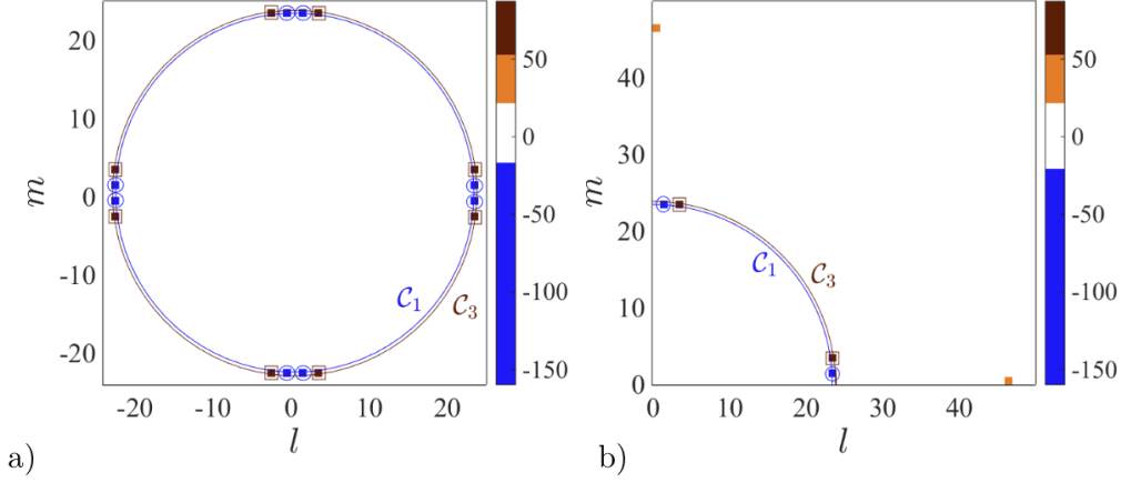
FIGURE 6. Spatial spectrum of a snapshot of the interface in the doubled domain. Circles \mathcal{C}_1 (dark blue) and \mathcal{C}_3 (dark brown) have slightly different radii. \mathcal{C}_1 contains the fundamental mode \hat{\zeta}_{23,1} and its images under reflection and rotation (dark blue dots surrounded by circles). \mathcal{C}_3 contains the highest third-harmonic mode \hat{\zeta}_{23,3} and its images (dark brown dots surrounded by squares). Only these modes and, to a lesser extent, the weaker second harmonic \hat{\zeta}_{46,0} (orange) have significant amplitude. a) Restriction to [-25, 25]^2 highlights the square symmetry of the pattern. b) Restriction to the first quadrant [0, 50]^2 includes \hat{\zeta}_{46,0} .
