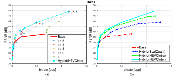
Fig. 4. RD curve of the base layer, local RD curves obtained for each lambda value and the RD curve obtained by computing the convex hull around all the point (a) and the comparison of the base layer and the improved versions (b) for the LF image Bikes .
