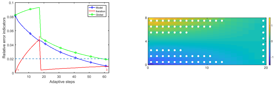
(a) Evolution of the error estimator and indicators along the adaptive process. (b) Map of the \epsilon_{yy} strain component for the final coupling solution.
