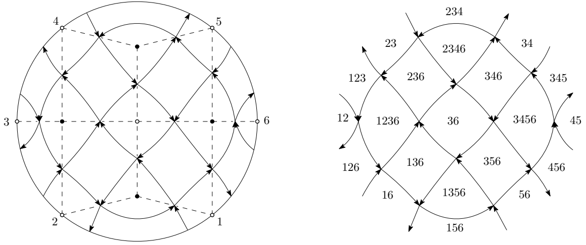
FIGURE 19. The alternating strand diagram for a plabic graph (left) and the associated labeling by sets of the faces and vertices of the graph (right).
