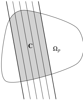
FIGURE 6.13. A constant zone in the case \#(I) = 2
