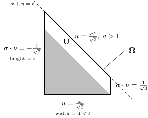
FIGURE 1. Example of non-uniqueness.
