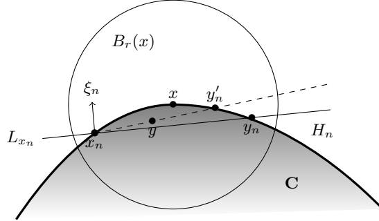
FIGURE 4. The case where x \in \partial\mathbf{C} \cap \partial\Omega_p is an accumulation point of (\partial\mathbf{C} \cap \partial\Omega_p) \setminus \partial^c\mathbf{C} , and x = \lim_n x_n = \lim_n y_n where x_n \notin \partial^c\mathbf{C} and x_n \neq y_n \in L_{x_n} \cap \partial\mathbf{C}
