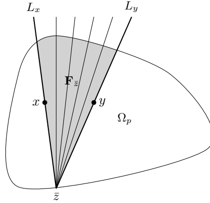
FIGURE 3. A boundary fan with apex \bar{z}
