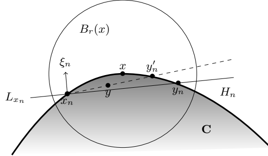
FIGURE 3. The case where x \in \partial \mathbf{C} \cap \partial \Omega_p is an accumulation point of (\partial \mathbf{C} \cap \partial \Omega_p) \setminus \partial^c \mathbf{C} , and x = \lim_n x_n = \lim_n y_n where x_n \notin \partial^c \mathbf{C} and x_n \neq y_n \in L_{x_n} \cap \partial \mathbf{C}
