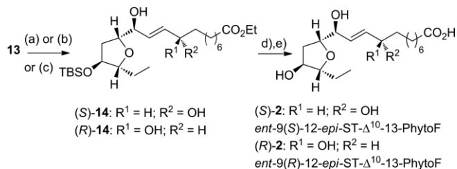
Scheme 4. (a) CeCl 3 ·7H 2 O, NaBH 4 , MeOH, 0 °C to r.t., 90 % for ( RS )- 14 , dr 1:1; (b) ( R )-methyl-CBS-oxazaborolidine, BH 3 ·Me 2 S, THF, 0 °C to r.t., 89 % for ( S )- 14 , dr 9:1; (c) ( S )-methyl-CBS-oxazaborolidine, BH 3 ·Me 2 S, THF, 0 °C to r.t., 76 % for ( R )- 14 , dr 9:1; (d) TBAF, THF, r.t.; (e) LiOH, THF/H 2 O, r.t.; 94 % for ( RS )- 2 ; 67 % for ( S )- 2 ; 90 % for ( R )- 2 over two steps. CBS: Corey–Bakshi–Shibata; TBAF: tetrabutylammonium fluoride.
