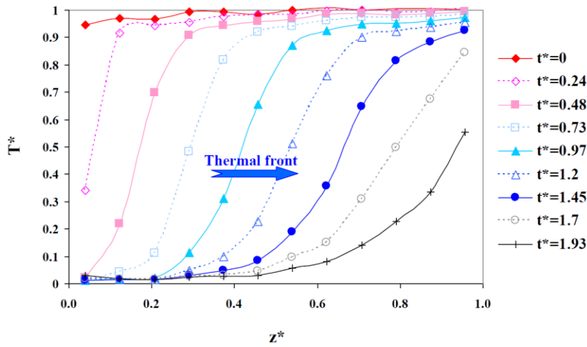
Fig. 6. Dimensionless fluid temperatures during discharge of a 2.4-m 3 packed bed of rocks and sand with thermal oil as HTF (Bruch et al., 2014b).
